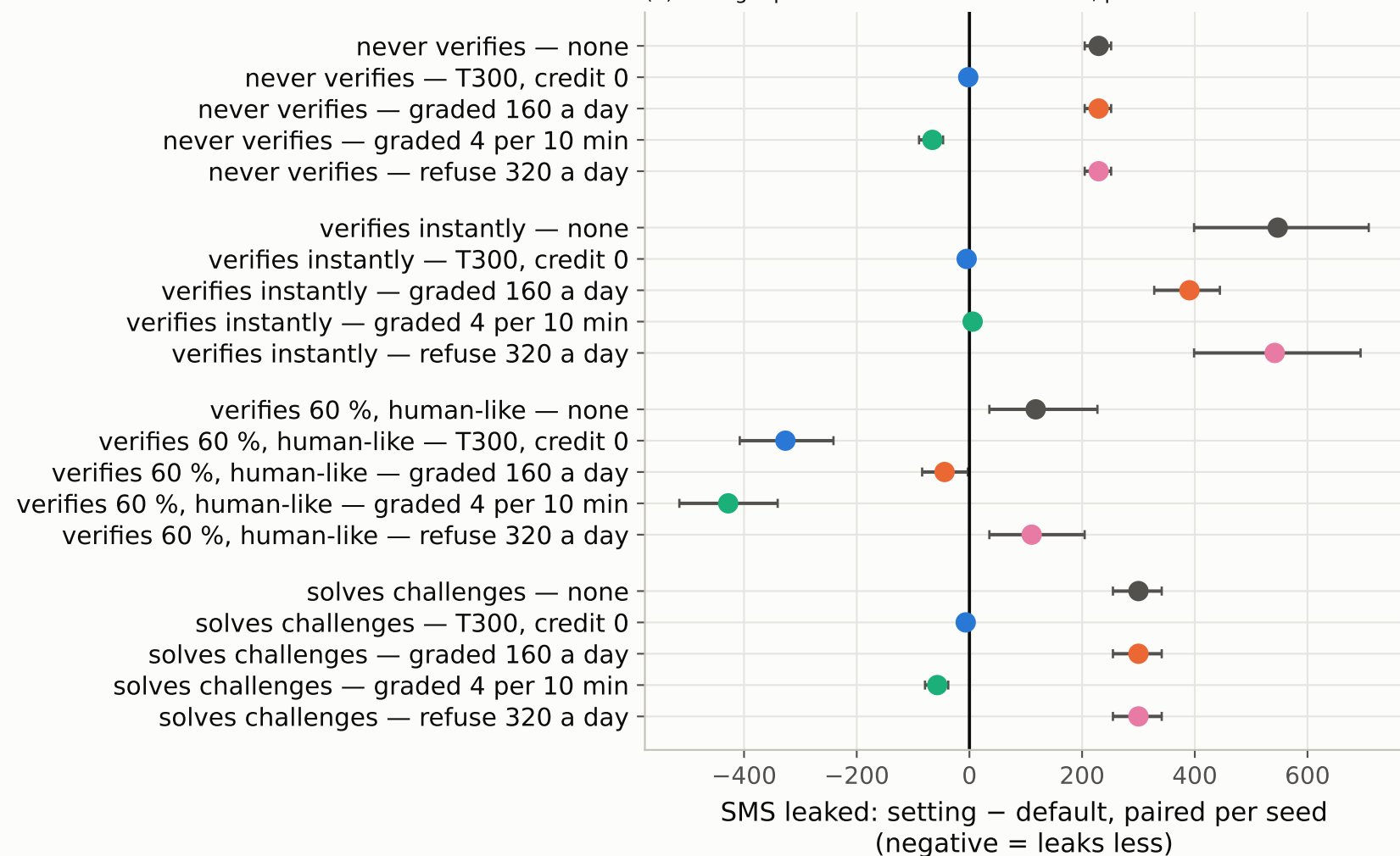
(b) leakage: paired difference to the default, per attacker
