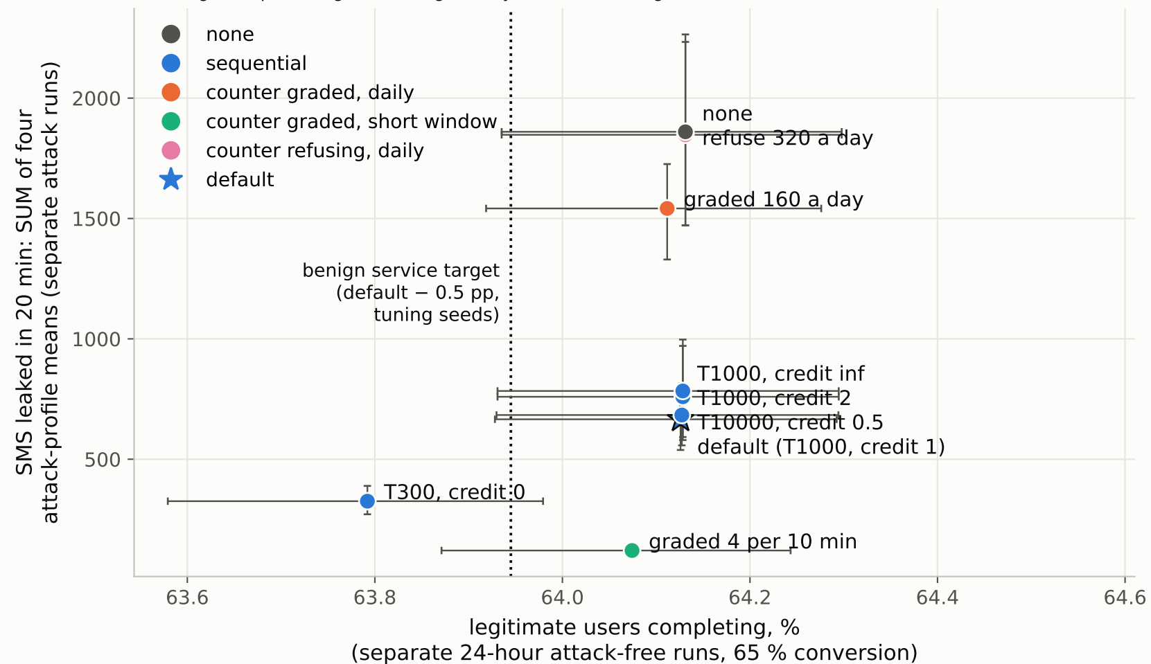
(a) benign completion against leakage, every evaluated setting
