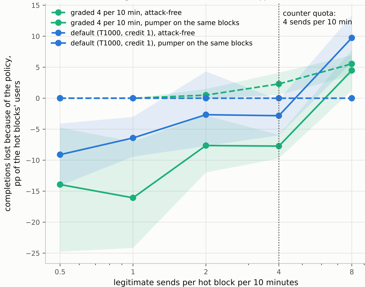
(a) service: loss among the hot blocks' users (70 % WhatsApp)
