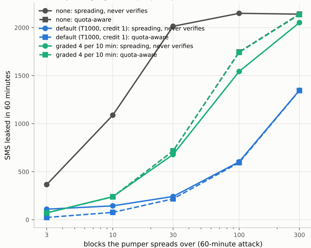
(b) security: leakage against the pumper's spread
