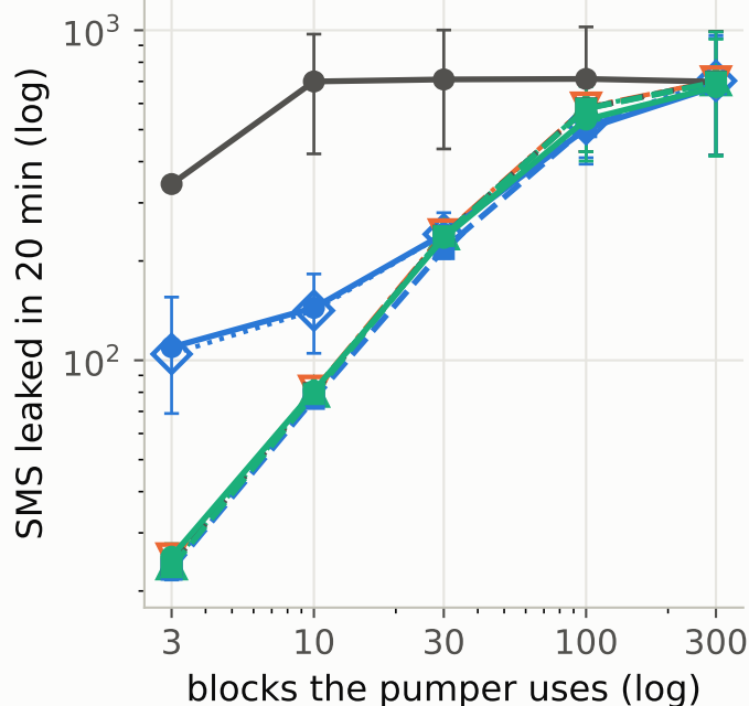
(b) security, 20-minute attack
