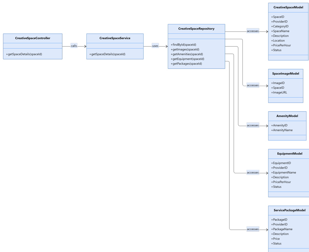
Class Diagram
