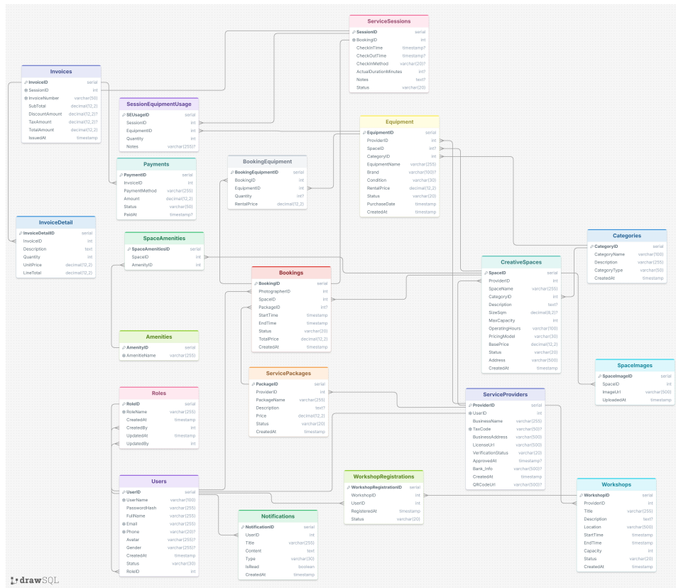
Figure IV.6: Entity Relationship Diagram
