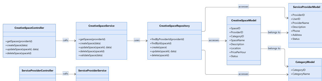
Class Diagram
