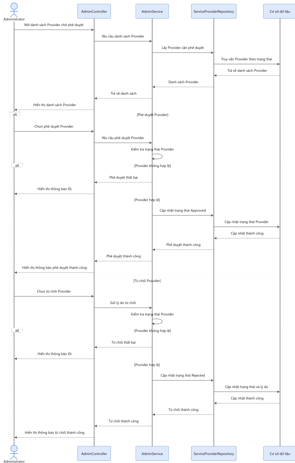
Sequence Diagram
