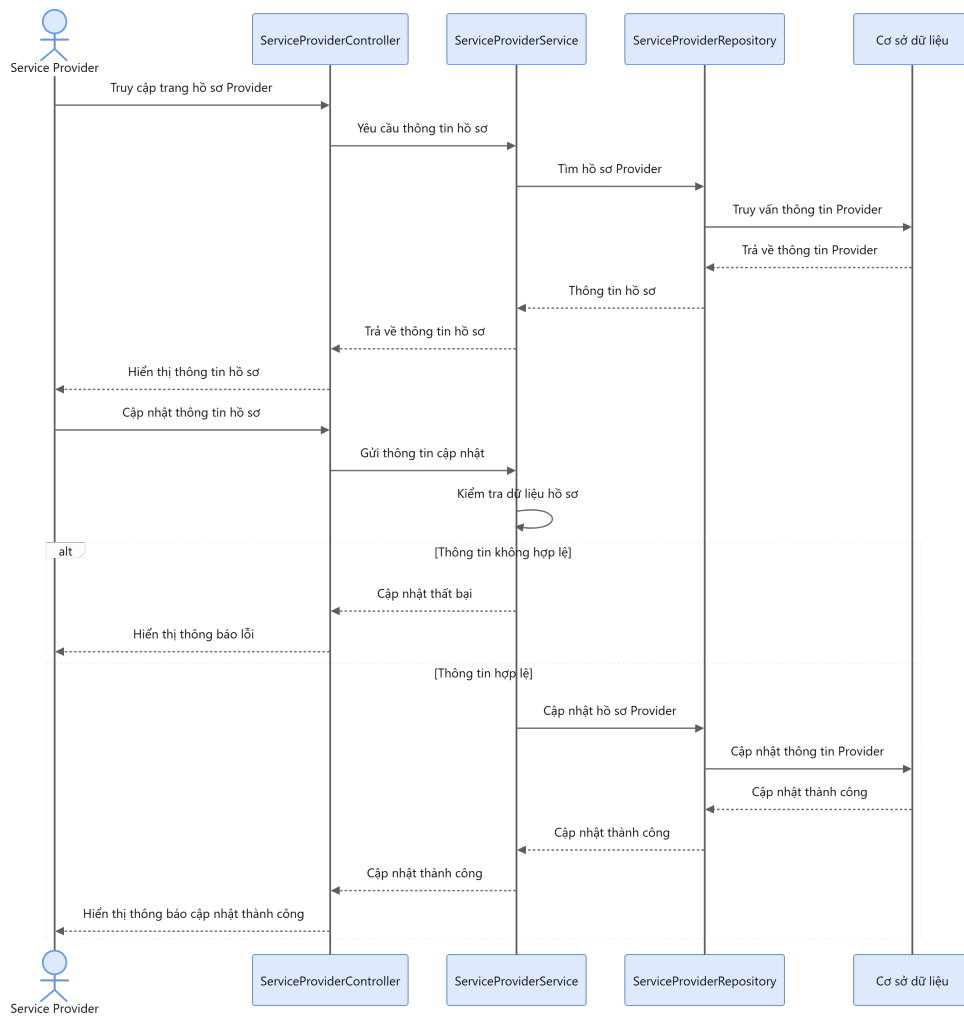
Sequence Diagram
