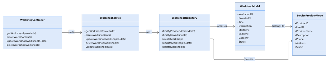
Class Diagram
