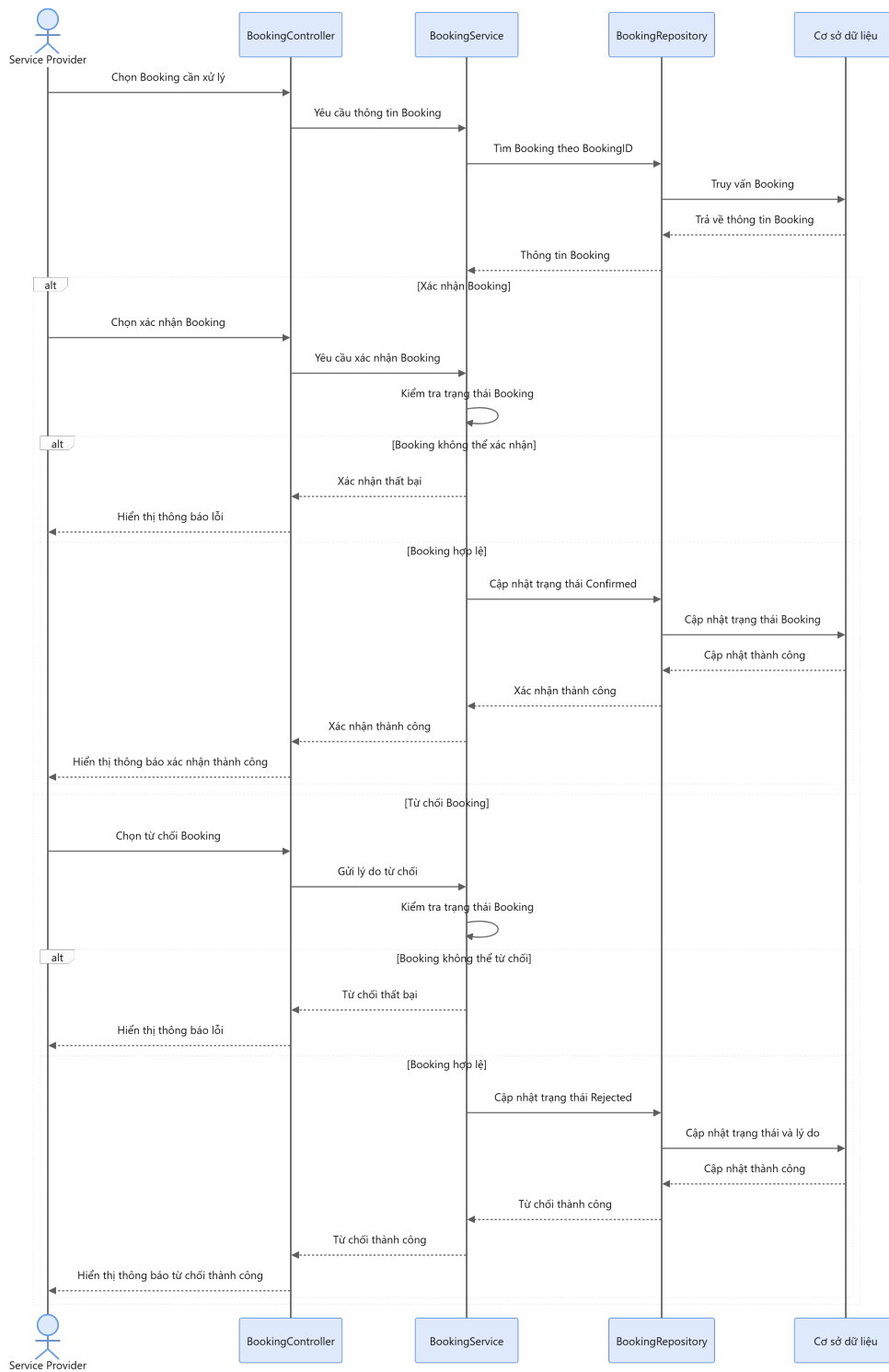
Sequence Diagram
