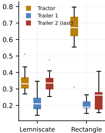
off-tracking of the estimated posture (m)
