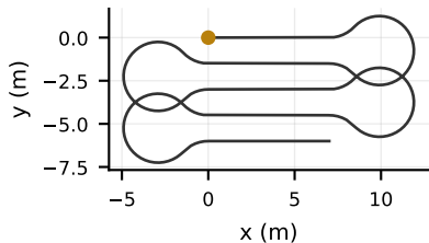
(a) agricultural: omega headland turns 86 m long, min radius 2.0 m
