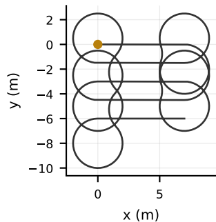
(a) agricultural: omega headland turns 128 m long, min radius 2.0 m
