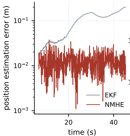
Bounded noise
