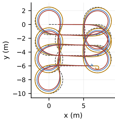
Pure pursuit (tractor)
