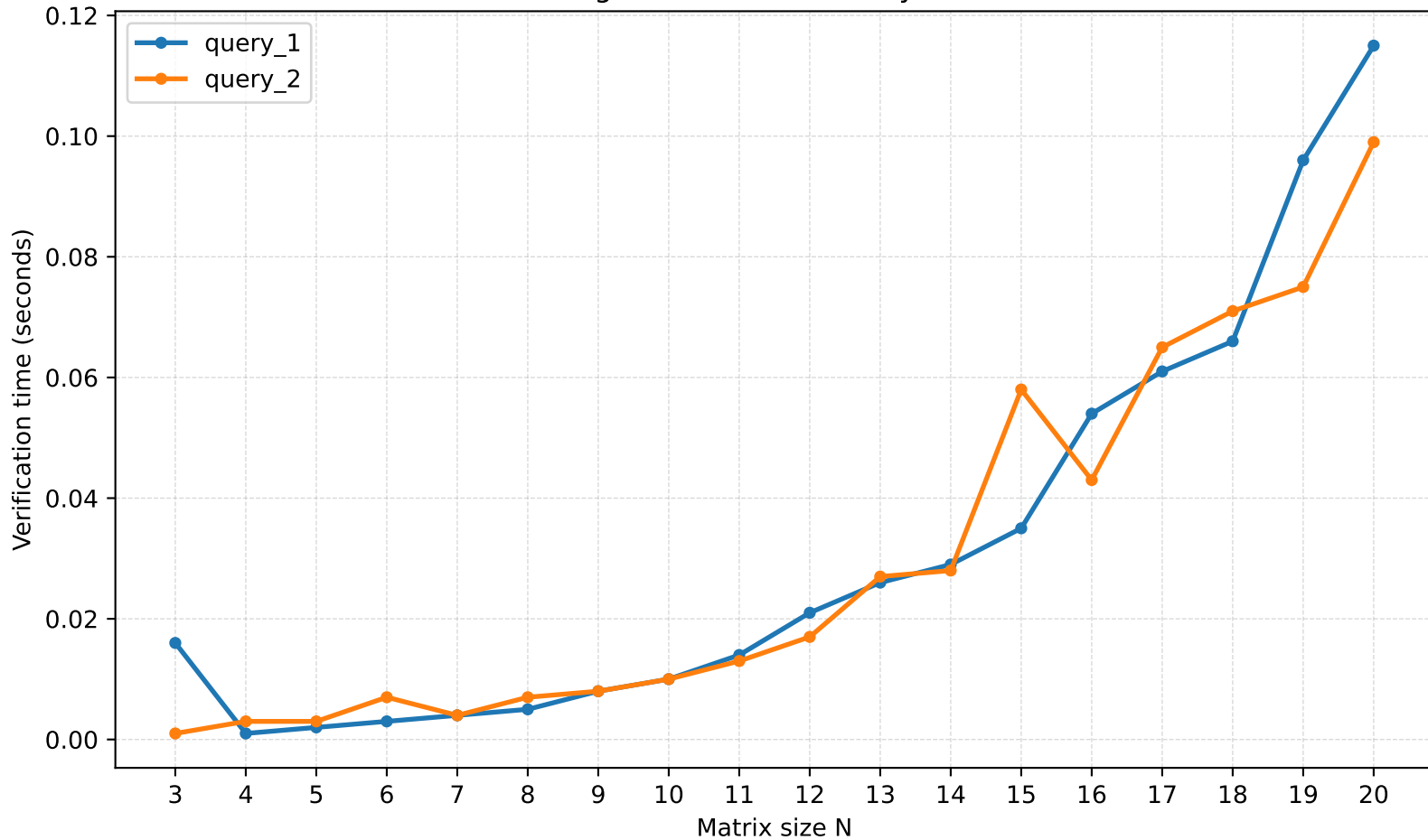
Verification Time vs Matrix Size Abstracted bvmul with ground commutativity axioms on observed calls
