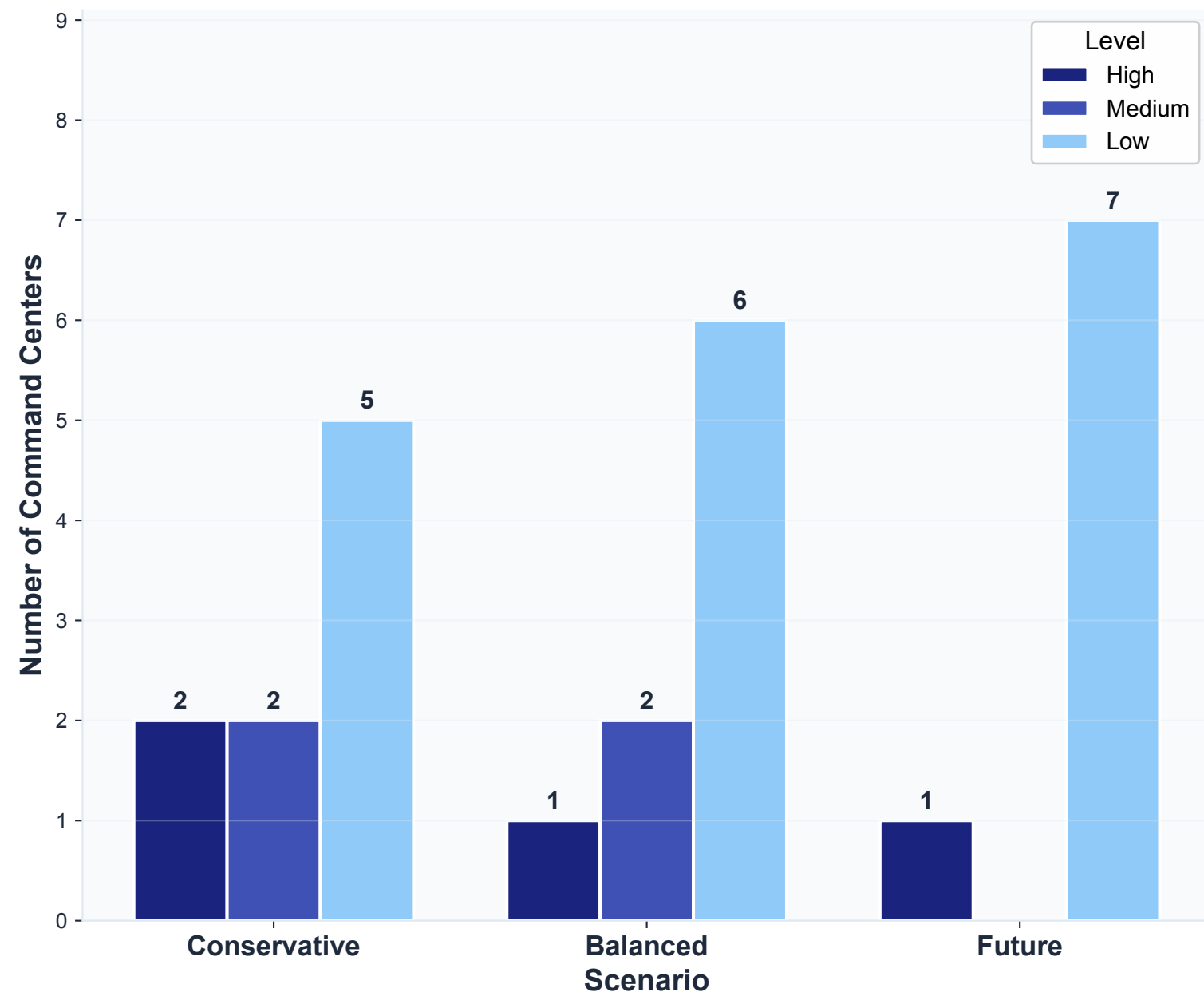
Heuristic Method
