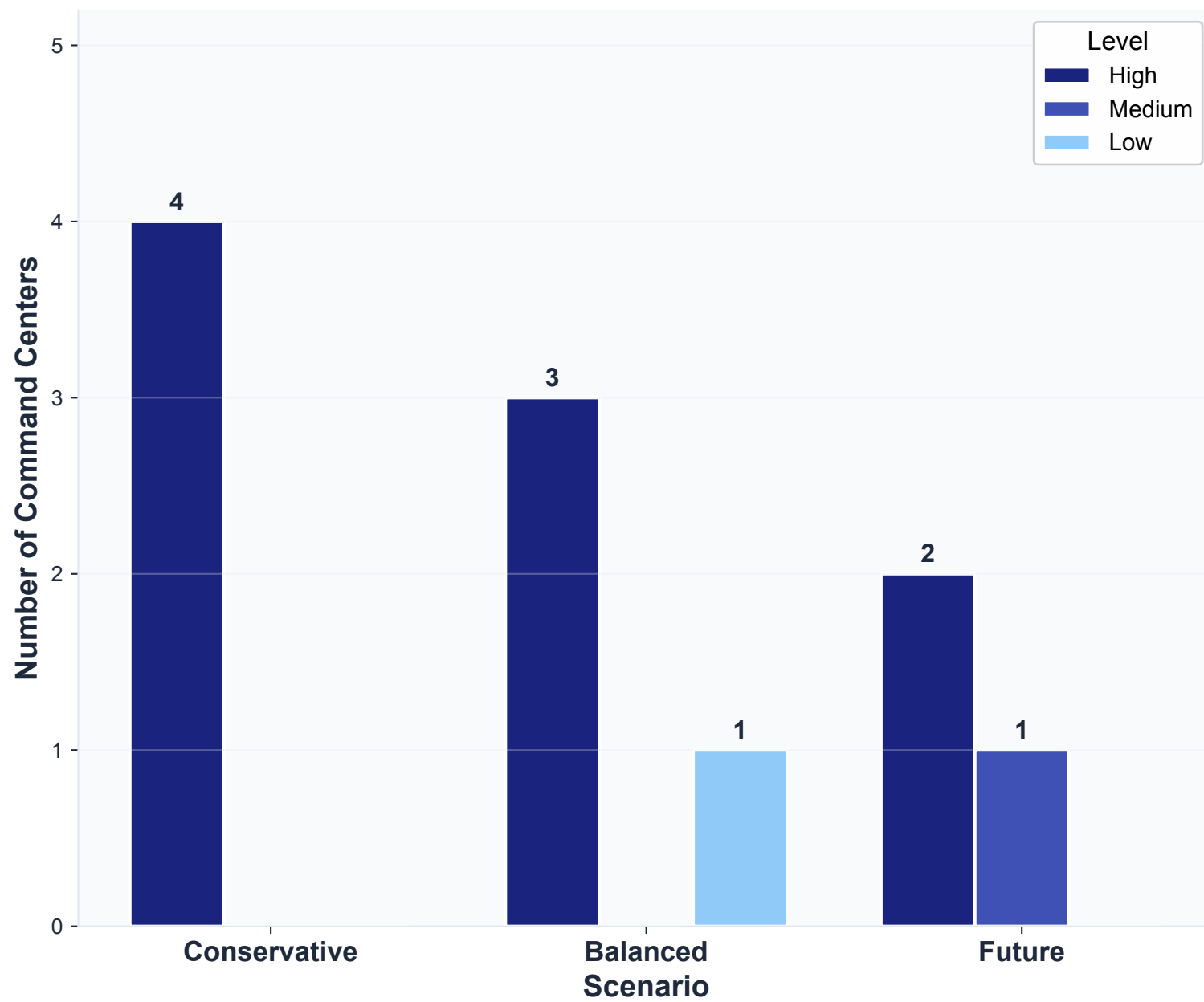
Exact Method
