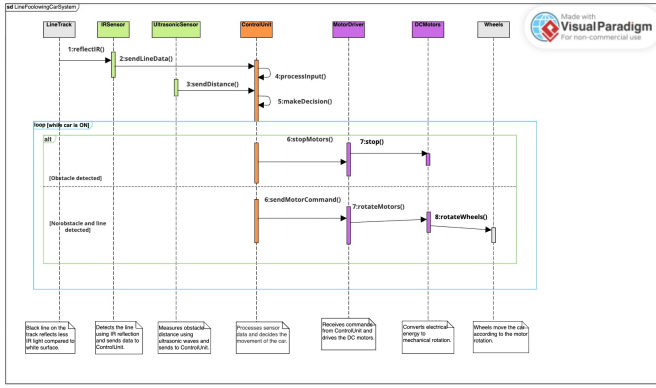
Fig. 4. Sequence Diagram
