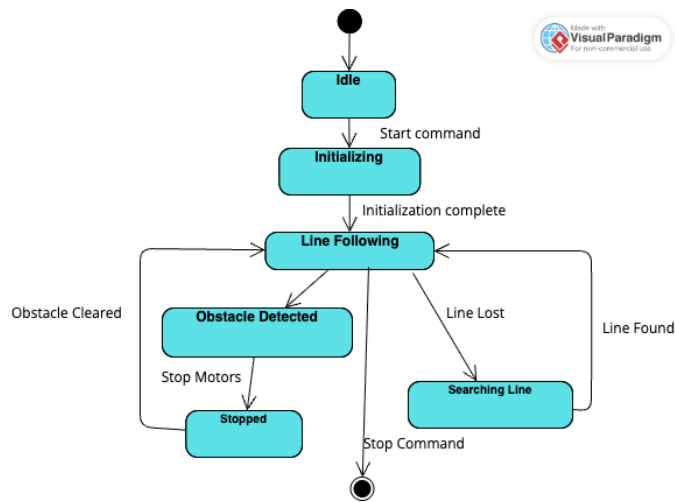
Fig. 6. State Machine Diagram
