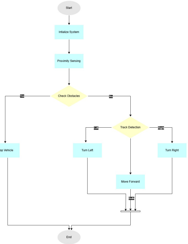
Fig. 3. Activity Diagram
