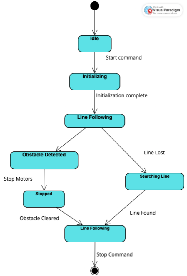
Fig. 6. State Machine Diagram
