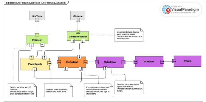
Fig. 2. Internal Block Diagram
