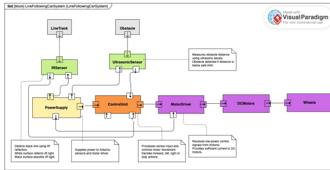
Fig. 2. Internal Block Diagram
