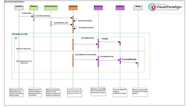
Fig. 4. Sequence Diagram
