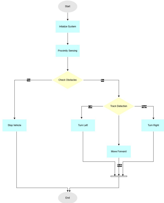
Fig. 3. Activity Diagram
