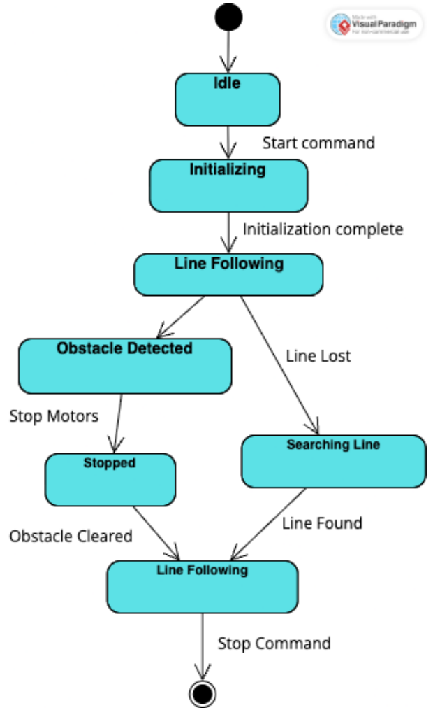
Fig. 6. State Machine Diagram
