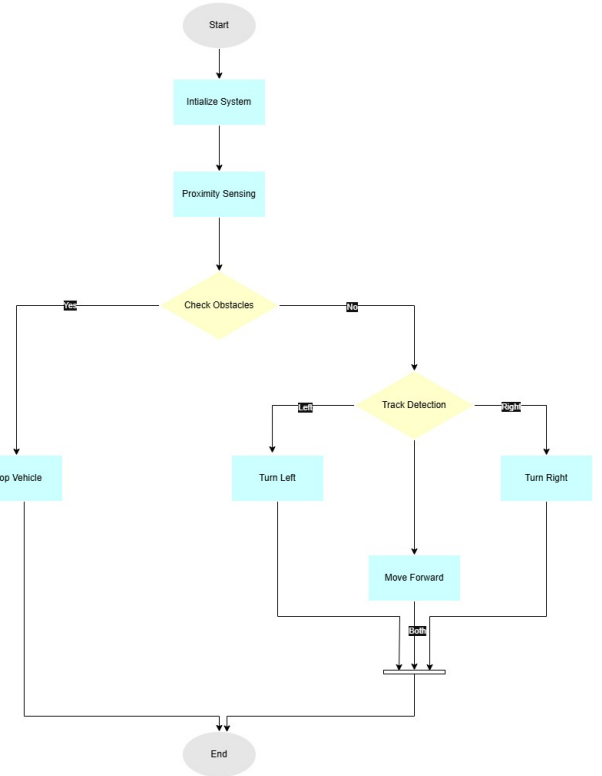
Fig. 3. Activity Diagram
