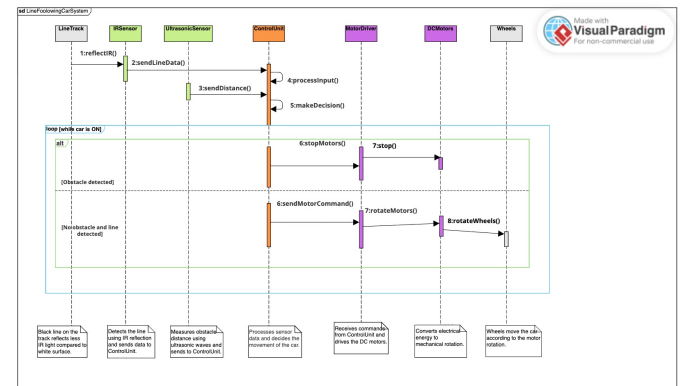
Fig. 4. Sequence Diagram
