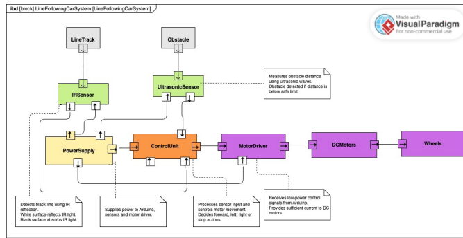
Fig. 2. Internal Block Diagram
