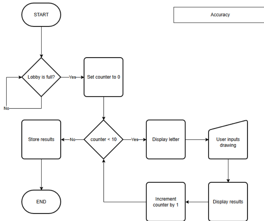
Figure 10: Accuracy flowchart
