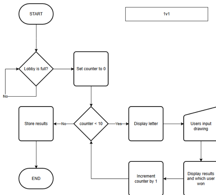
Figure 11: Versus flowchart
