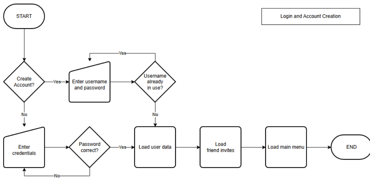
Figure 9: Account flowchart
