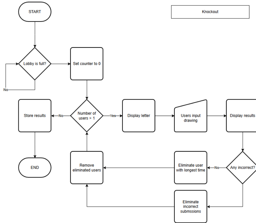
Figure 12: Knockout flowchart
