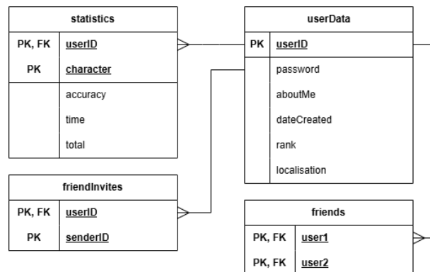
Figure 13: Entity-Relationship diagram
