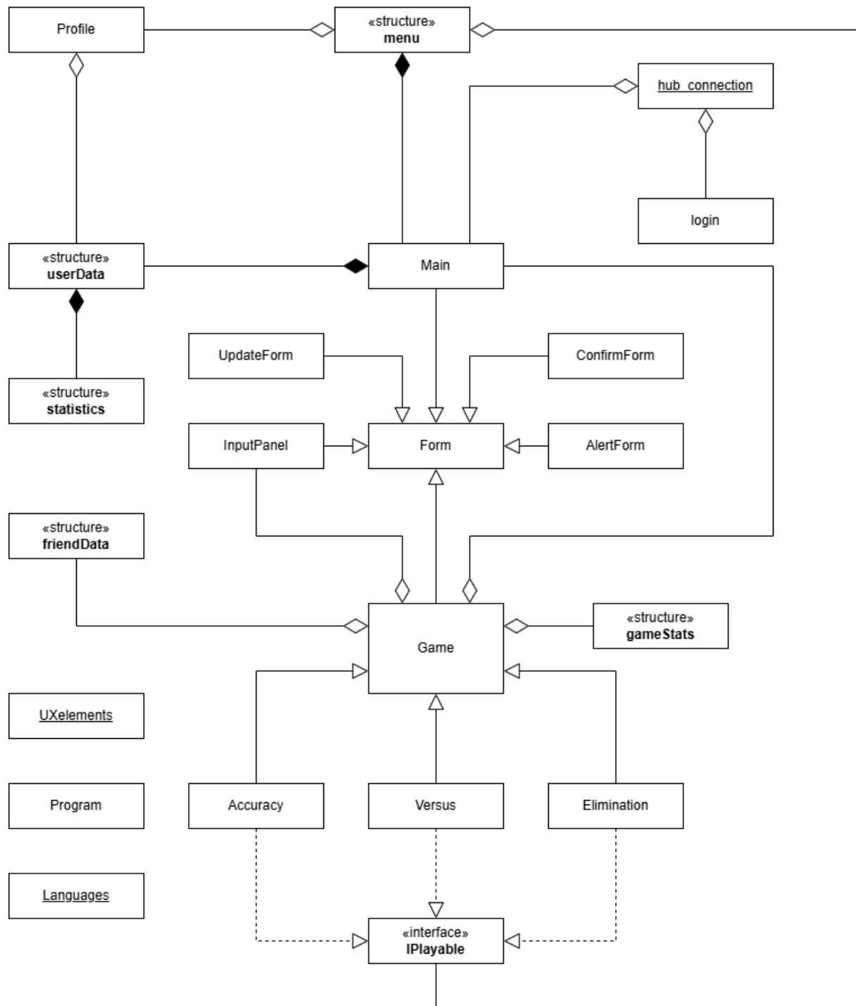
Figure 38: Relationships between the client classes
