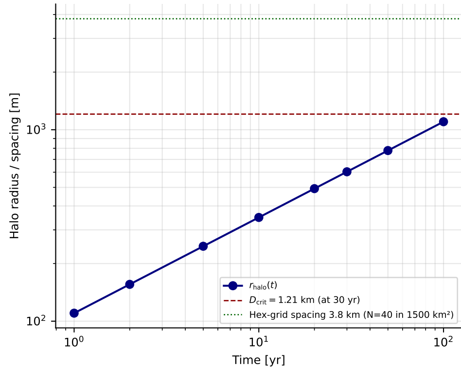
Single-doublet thermal halo growth
