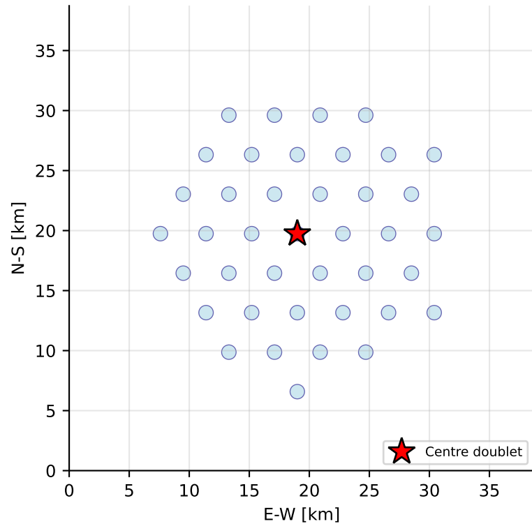
N=40 doublets on 3.8 km hex grid ( 1500 \text{ km}^2 ) + 30-yr thermal halos ( r=603 \text{ m} ). Halos do not touch.
