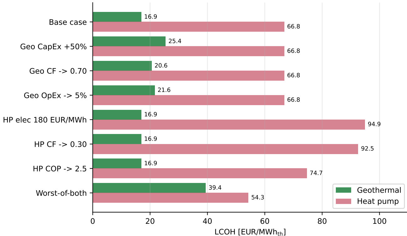
Levelised cost of heat: geothermal vs.\ heat pump (deep Vienna Basin doublet vs.\ Ebswien wastewater HP)
