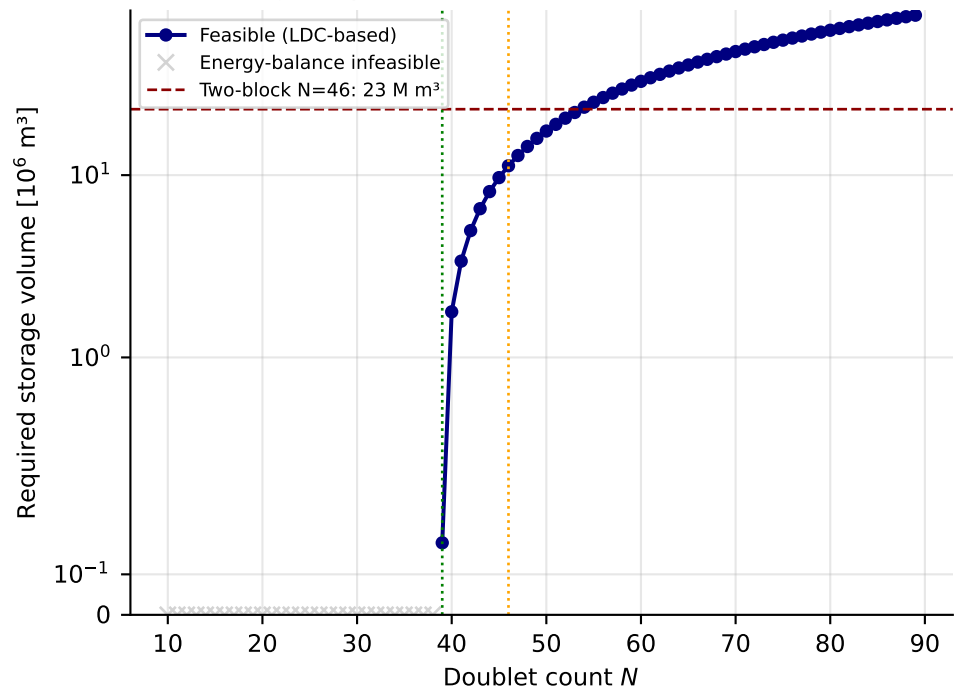
Storage requirement vs N (eta=0.70, deltaT=60 K)
