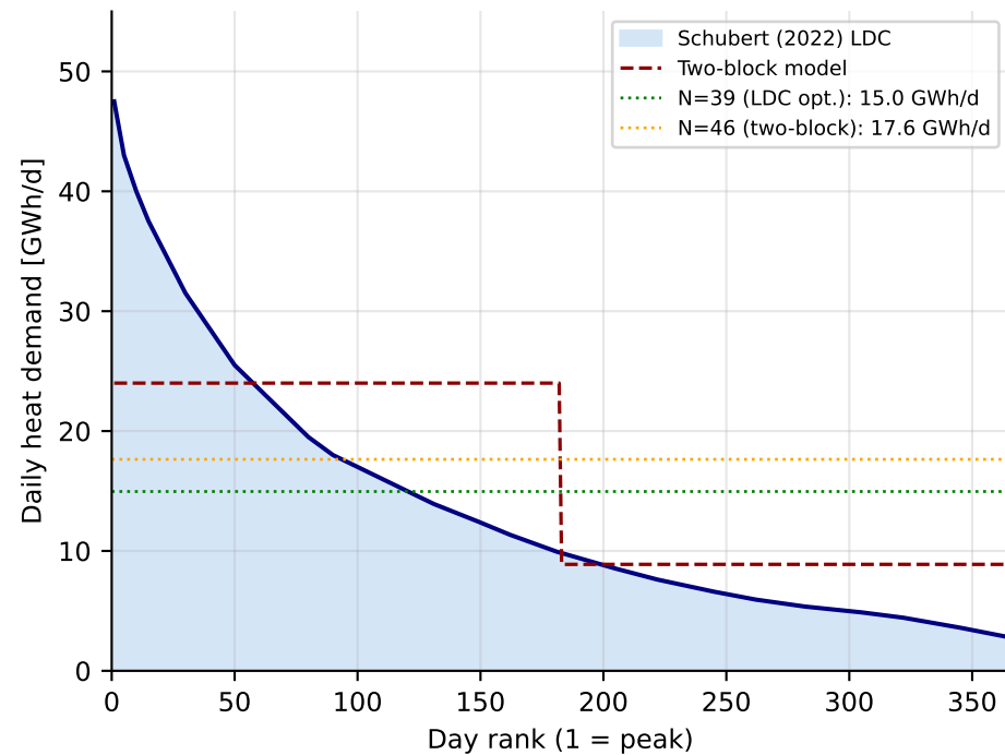
Load duration curve (Schubert 2022, Vienna 2040 scenario)
