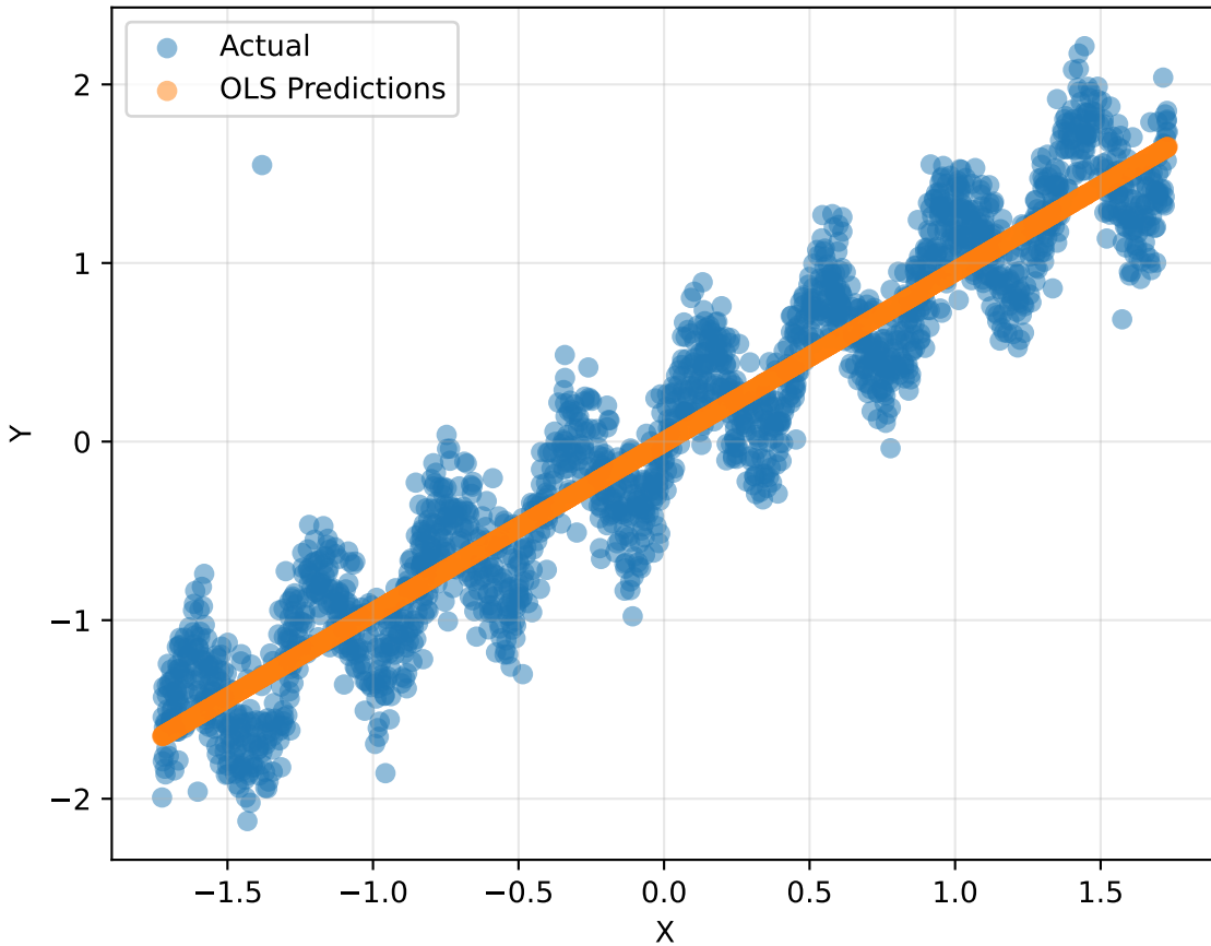
OLS Model Predictions
