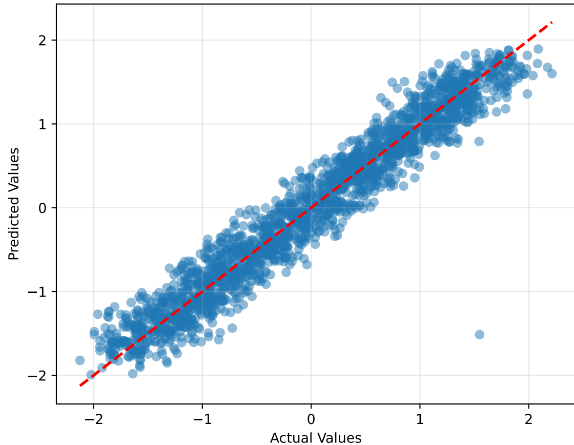
AI Model ( R^2 = 0.9406 )
