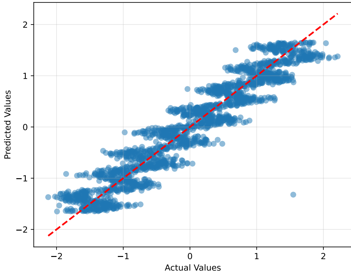
OLS Model ( R^2 = 0.9041 )
