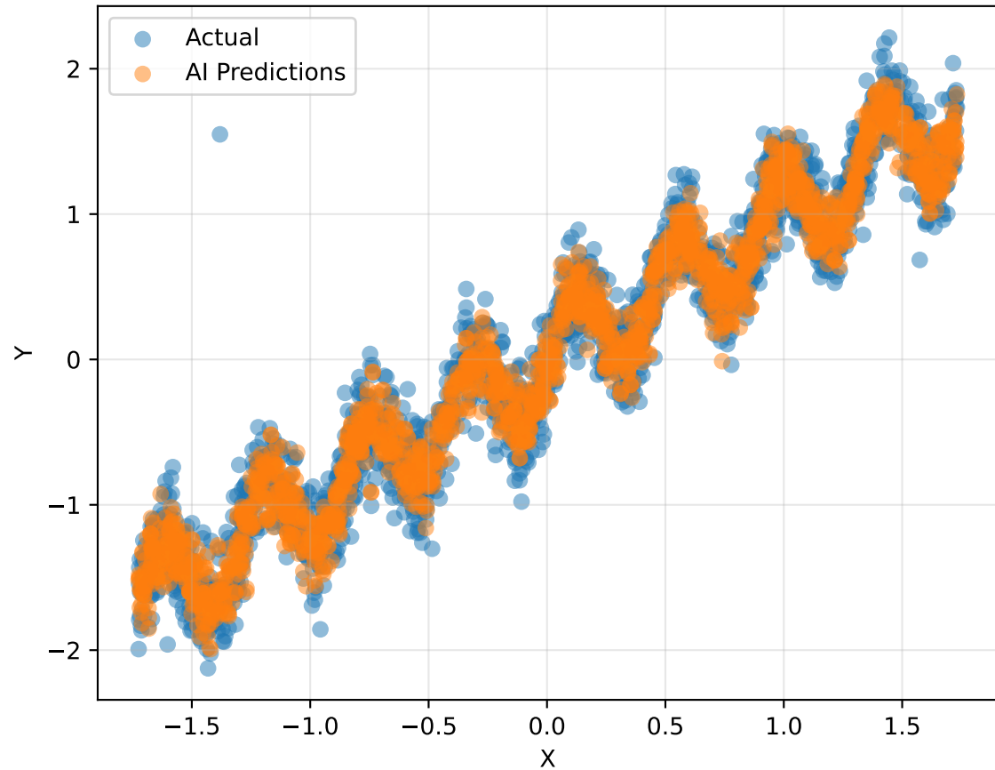
AI Model Predictions
