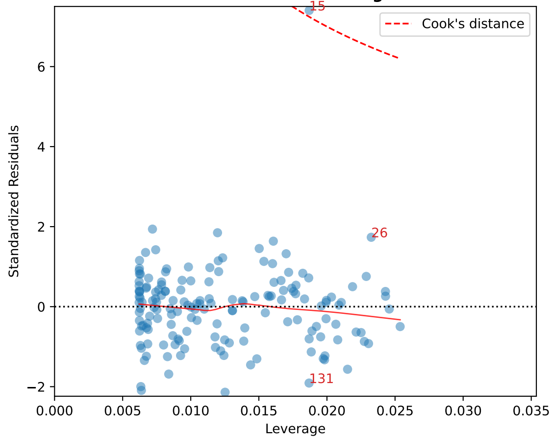
Residuals vs Leverage
