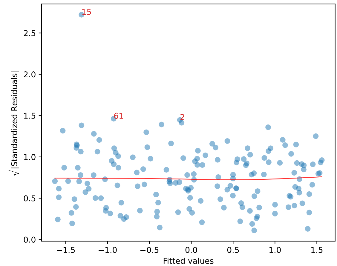
Scale-Location
