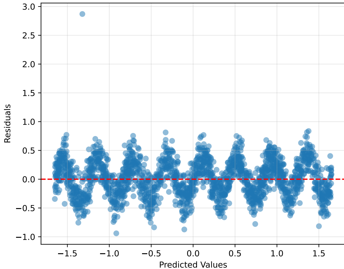
OLS Model Residuals
