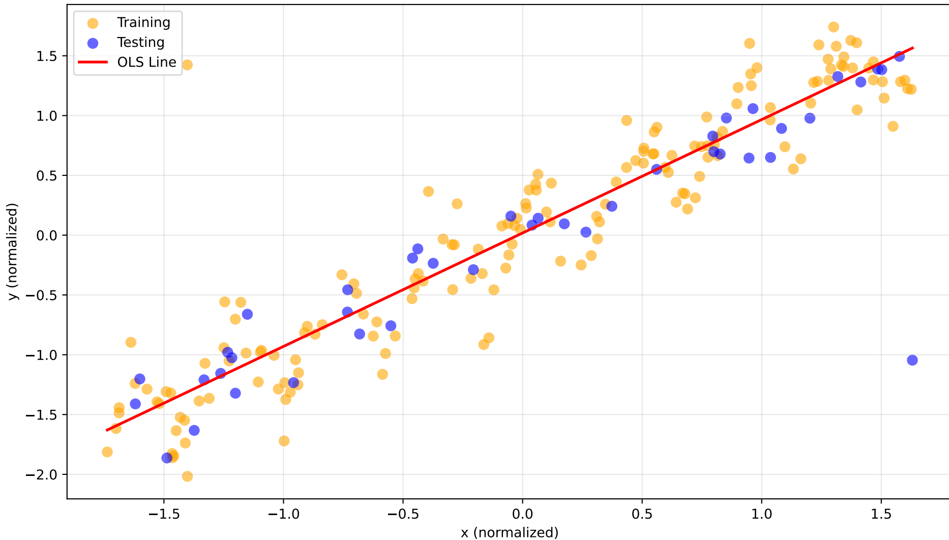
Scatter Plot with OLS Regression Line
