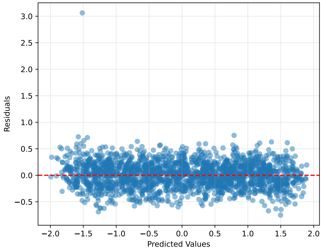
AI Model Residuals
