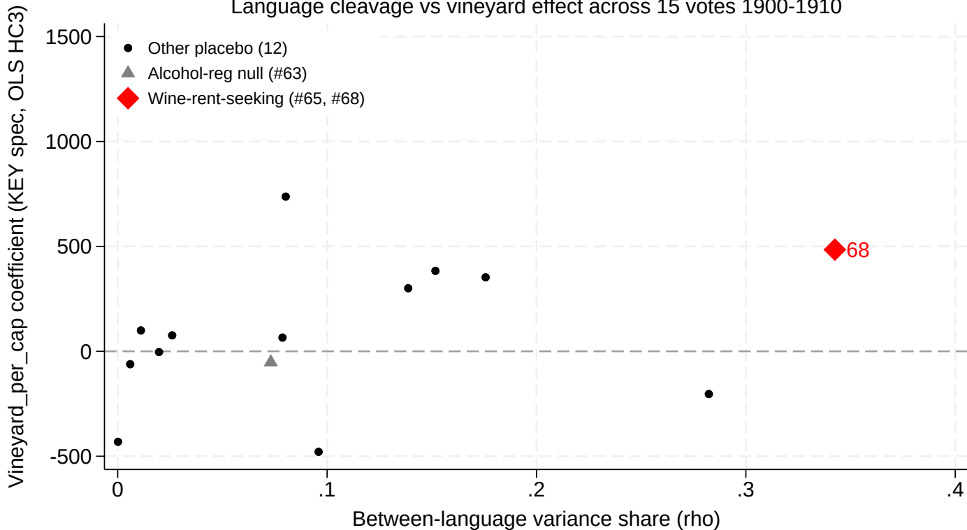
Language cleavage vs vineyard effect across 15 votes 1900-1910
