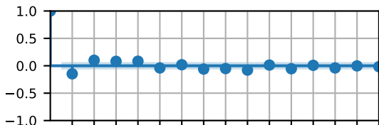
Differenced flux PACF
