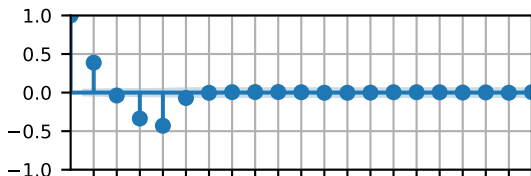
Differenced flux ACF
