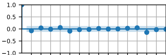
Residual PACF
