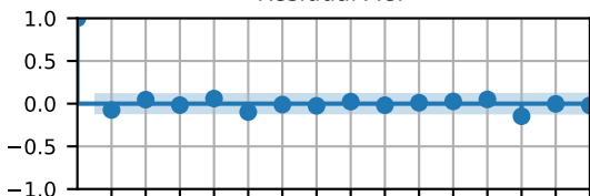
Residual ACF
