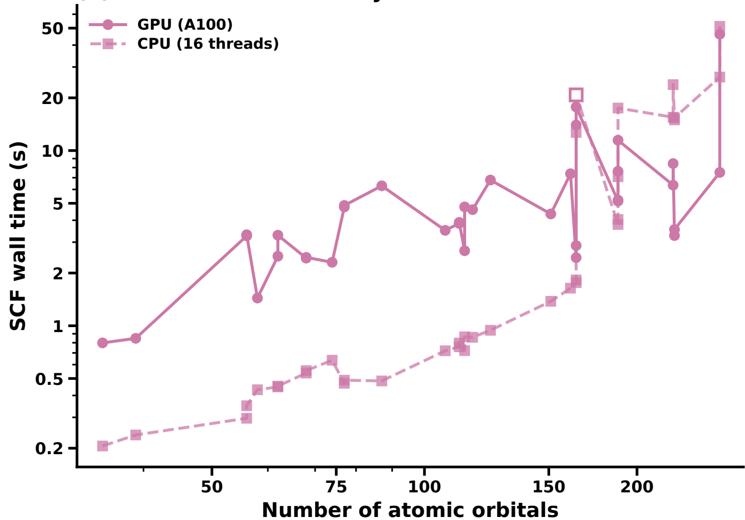
(a) B3LYP wall time vs system size
