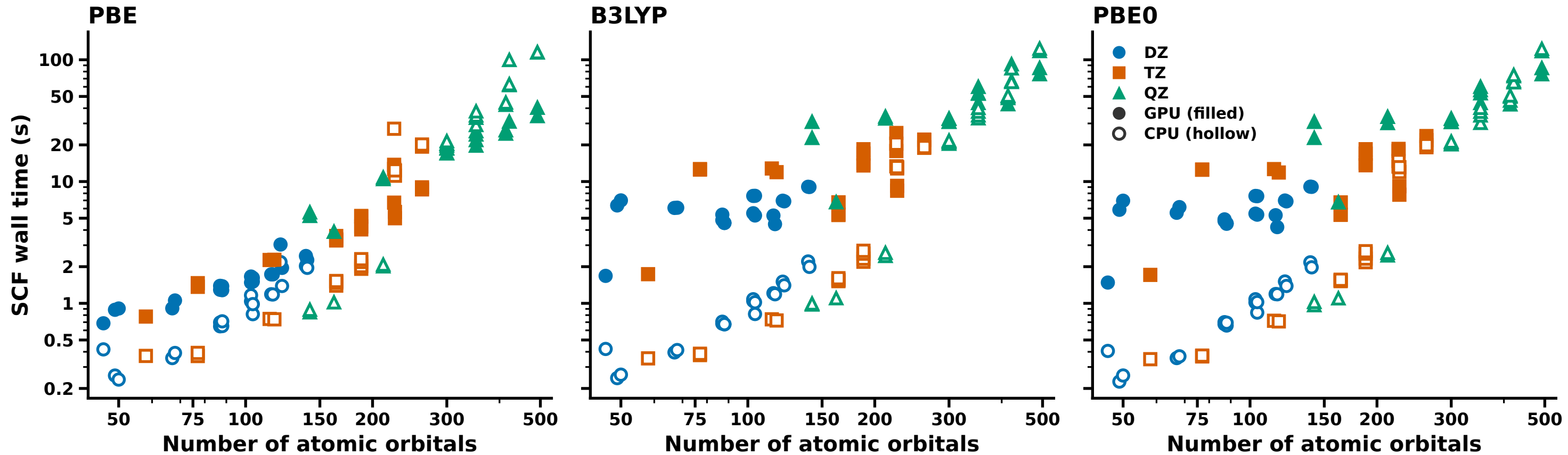
(b) SCF wall time vs system size, GPU and CPU
