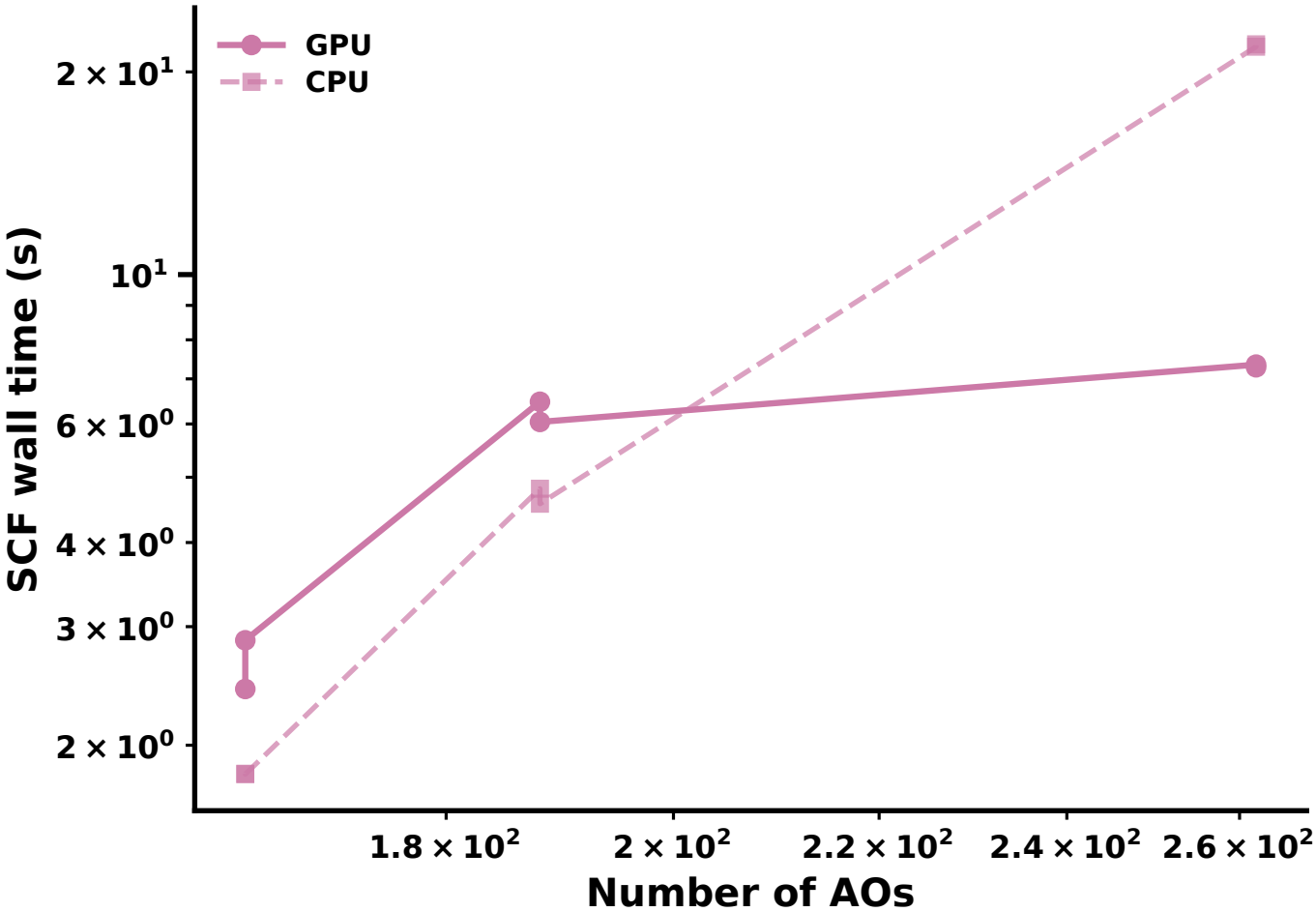
(a) B3LYP wall time vs system size solid = GPU, dashed = CPU
