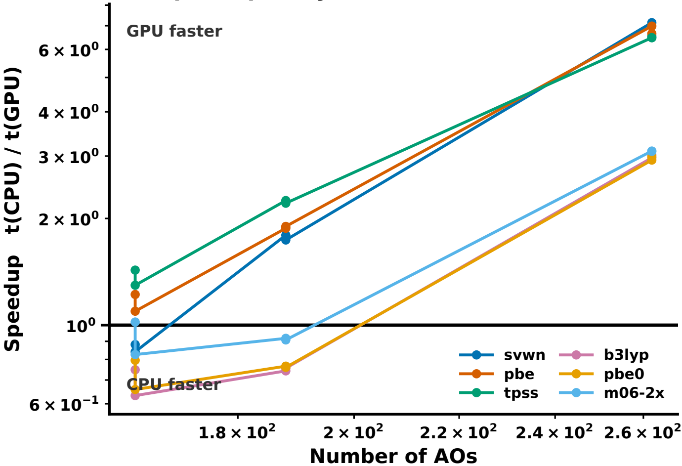
(b) Speedup vs system size
