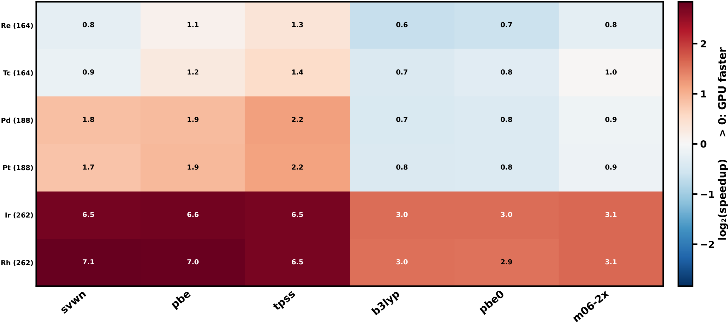
(c) Speedup by element (AO count) and functional
