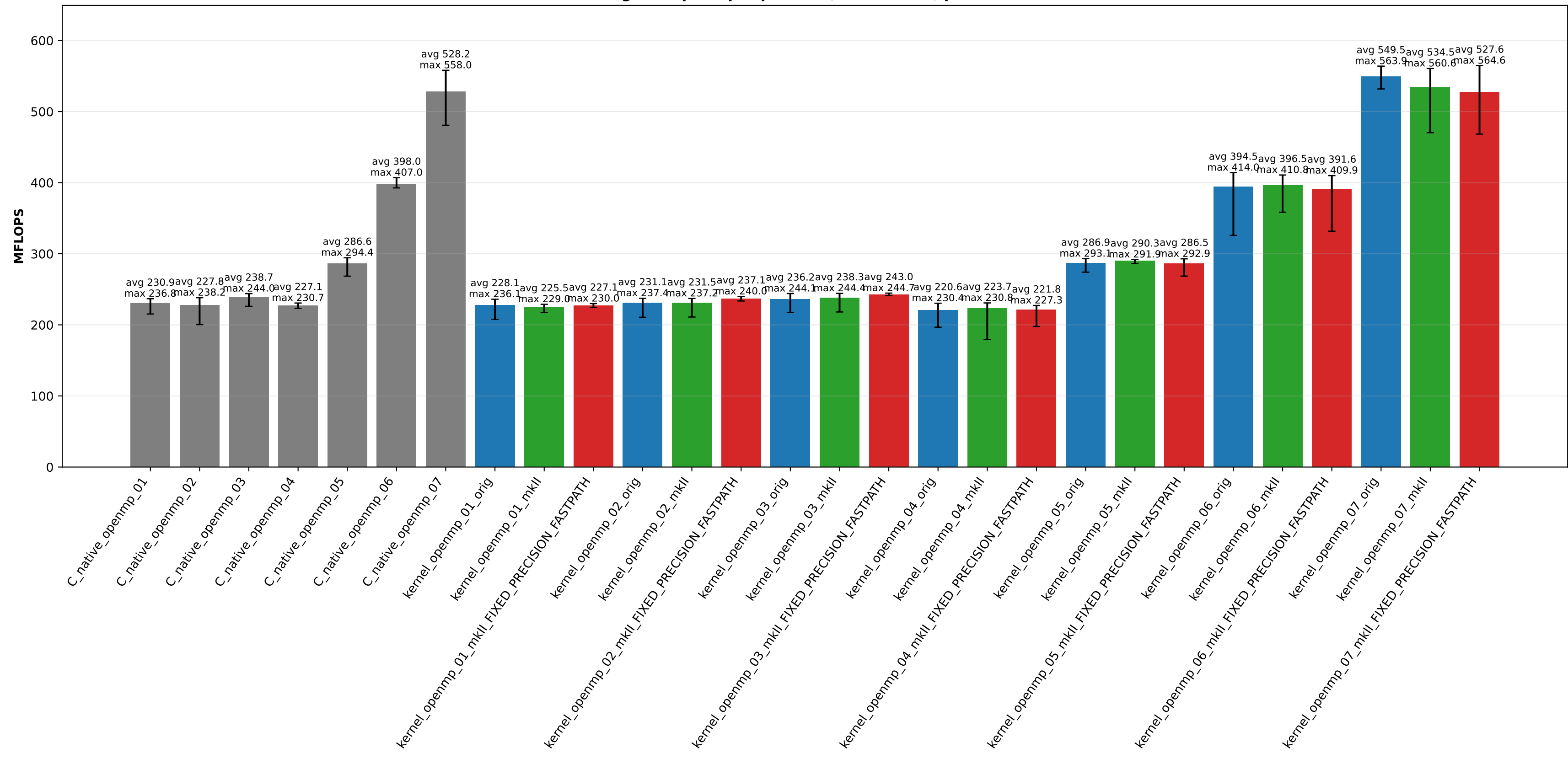
GMP Rgemv openmp repeat=10, M=N=4000, precision=512
