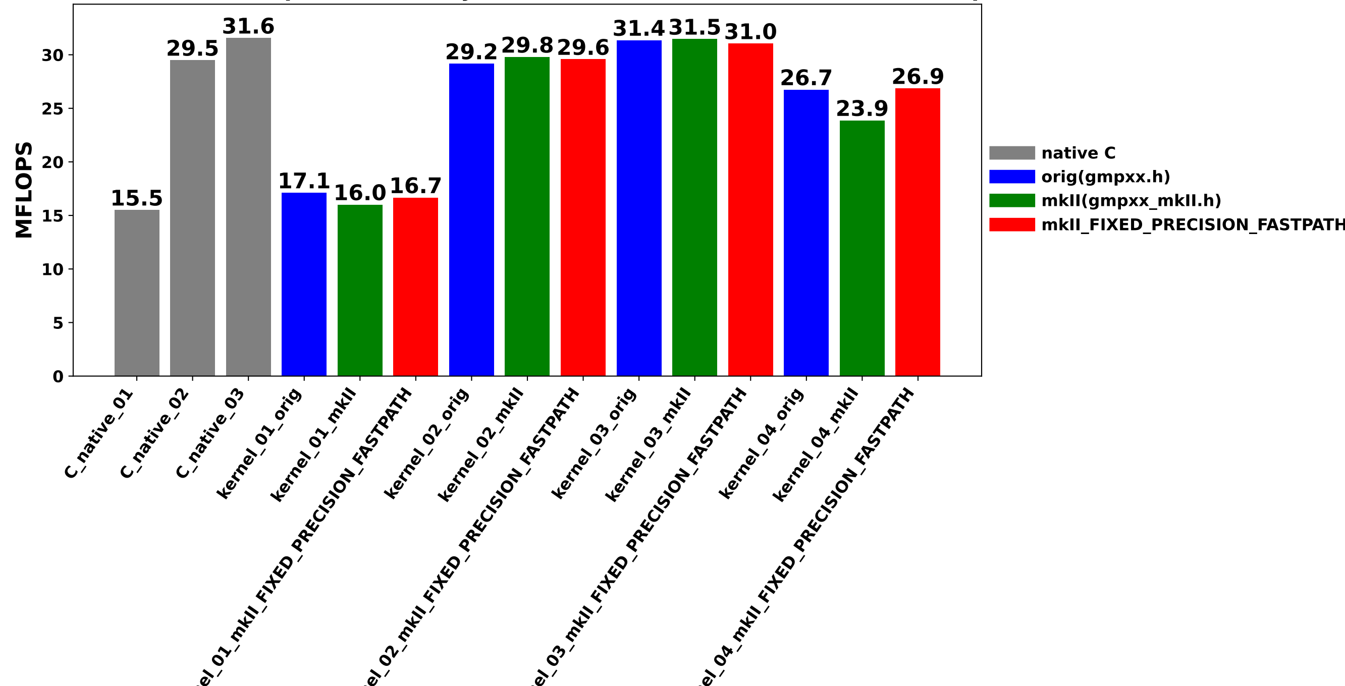
MFLOPS for Various GMP Operations on Ryzen 3970X 32-Core (dim=(4,000, 4,000), prec=512)
