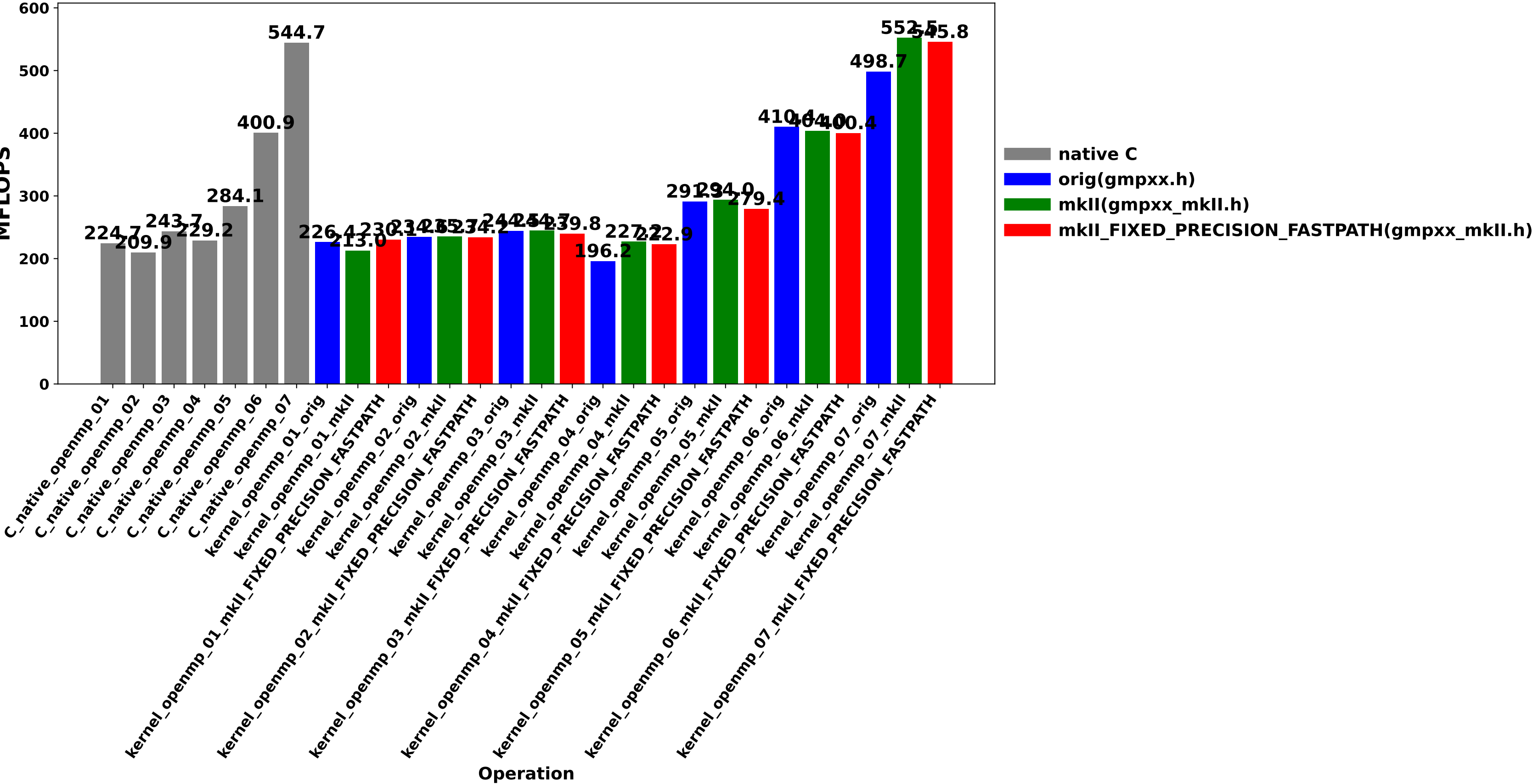
MFLOPS for OpenMP GMP Operations on Ryzen 3970X 32-Core (dim=(4,000, 4,000), prec=512)
