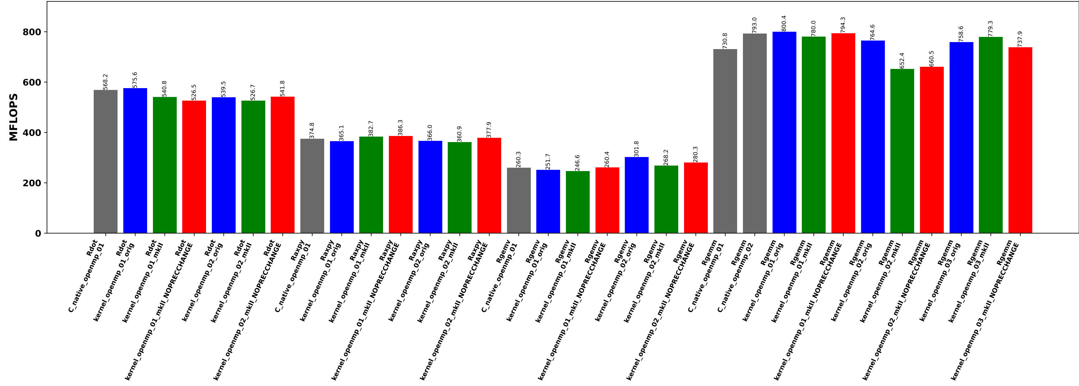
GMP OpenMP benchmark summary on Ryzen 3970X 32-Core (prec=512)
