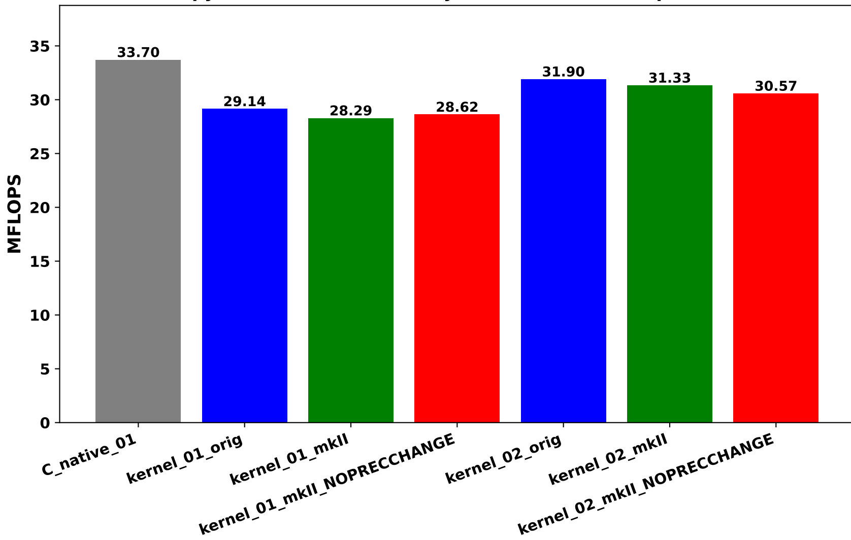
Raxpy serial benchmark on Ryzen 3970X 32-Core (prec=512)
