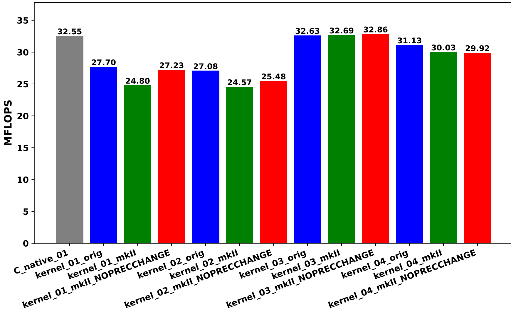
Rdot serial benchmark on Ryzen 3970X 32-Core (prec=512)
