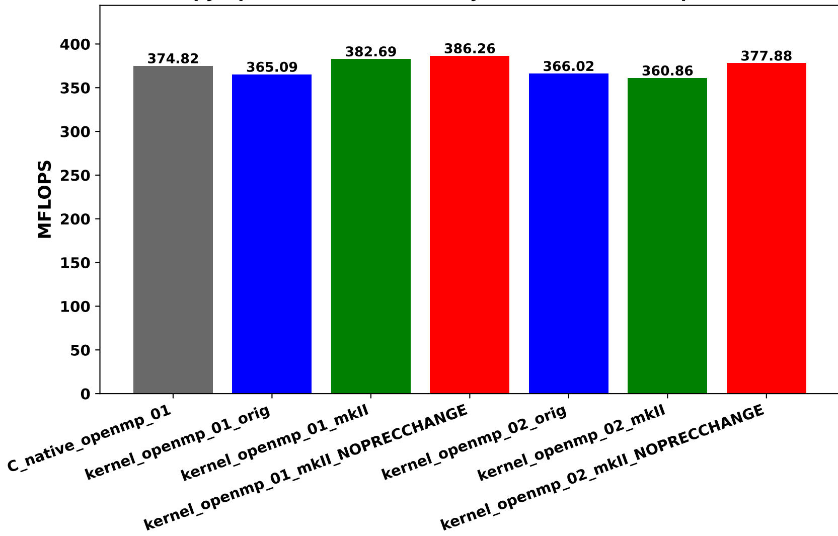
Raxpy OpenMP benchmark on Ryzen 3970X 32-Core (prec=512)
