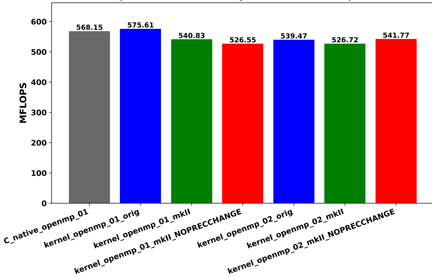
Rdot OpenMP benchmark on Ryzen 3970X 32-Core (prec=512)
