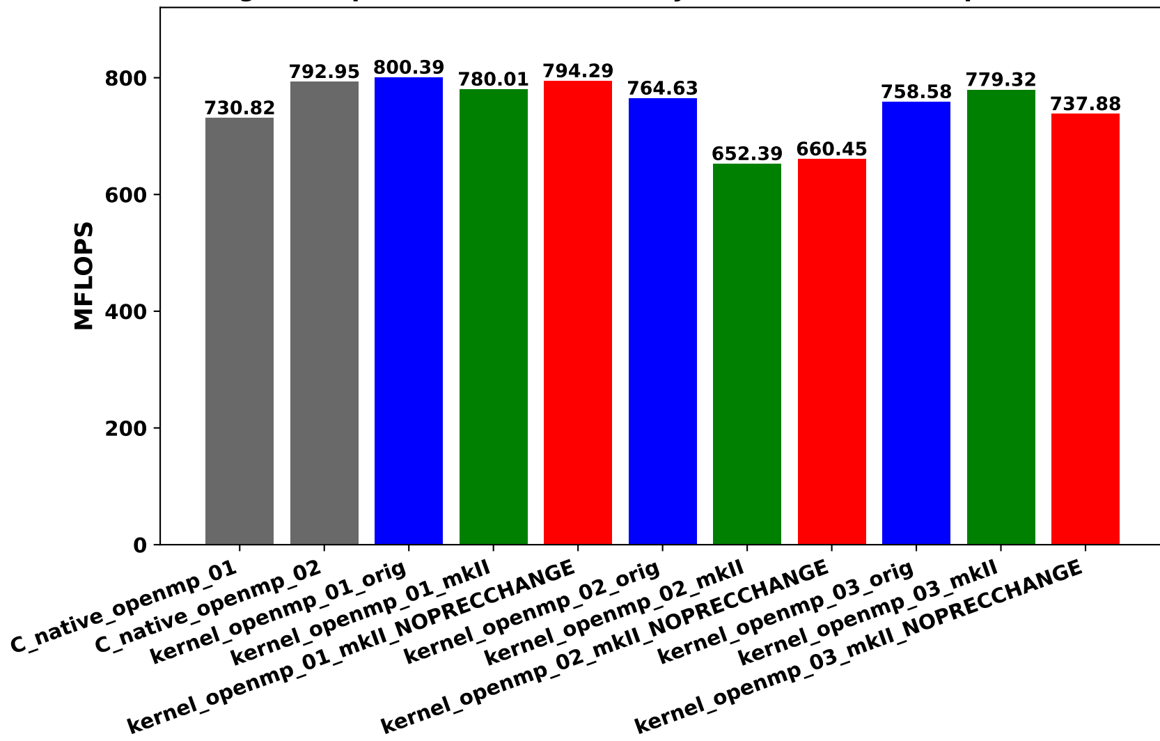
Rgemm OpenMP benchmark on Ryzen 3970X 32-Core (prec=512)
