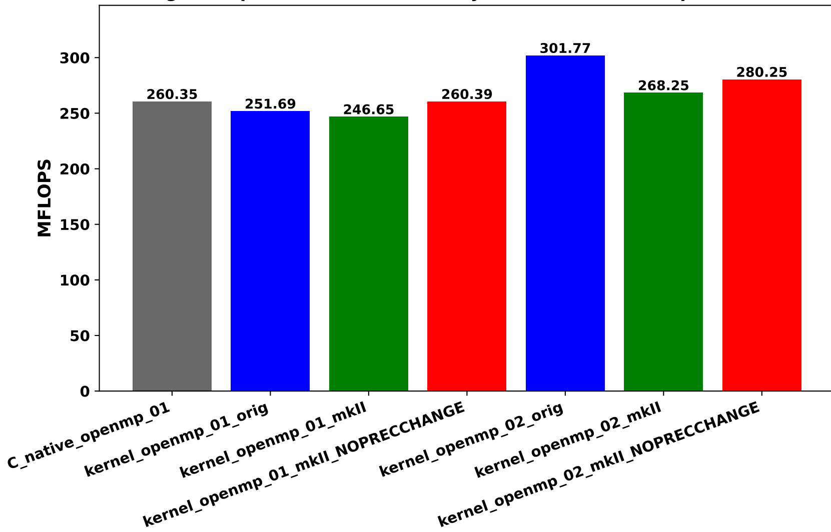
Rgemv OpenMP benchmark on Ryzen 3970X 32-Core (prec=512)
