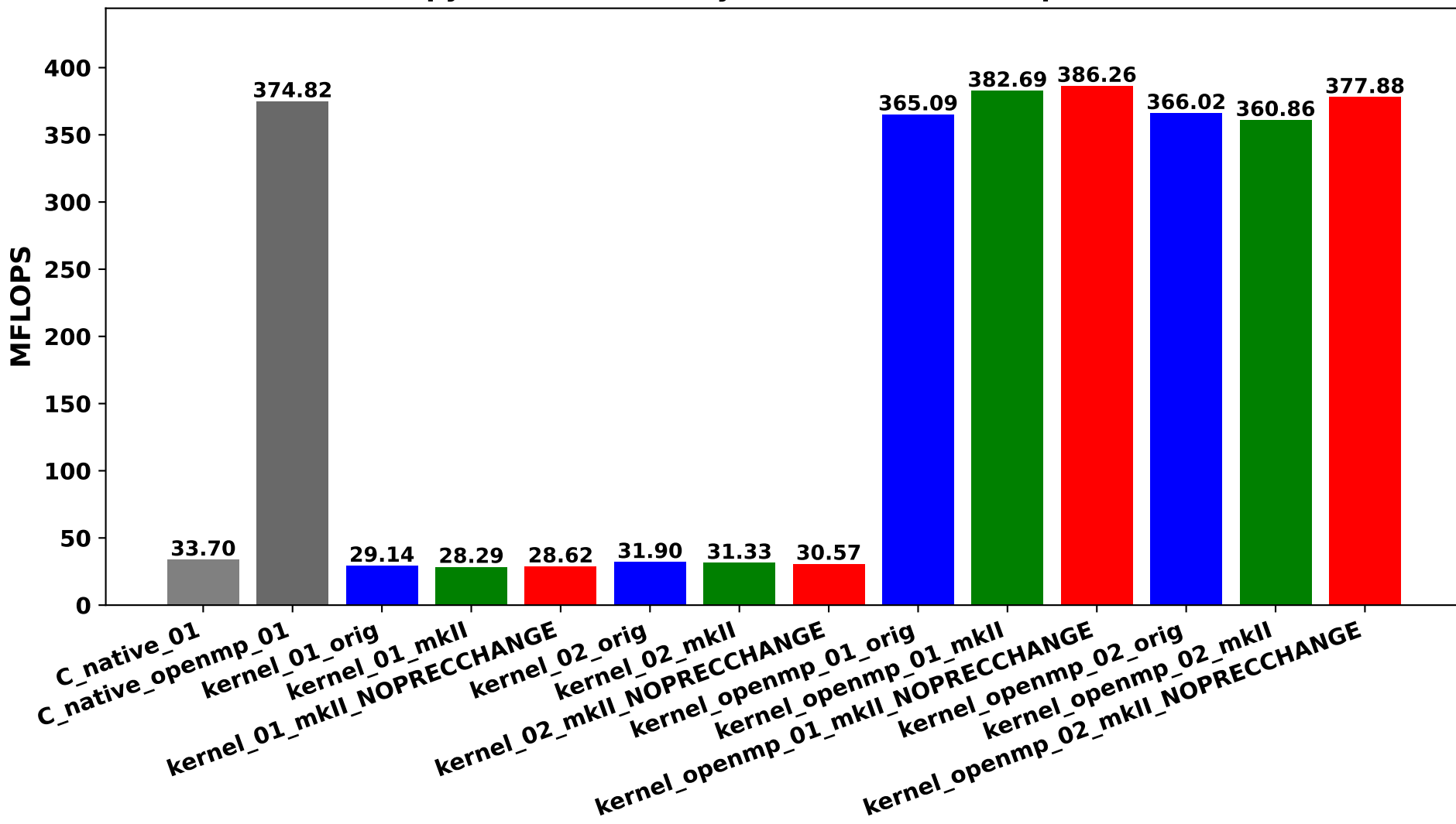
Raxpy benchmark on Ryzen 3970X 32-Core (prec=512)
