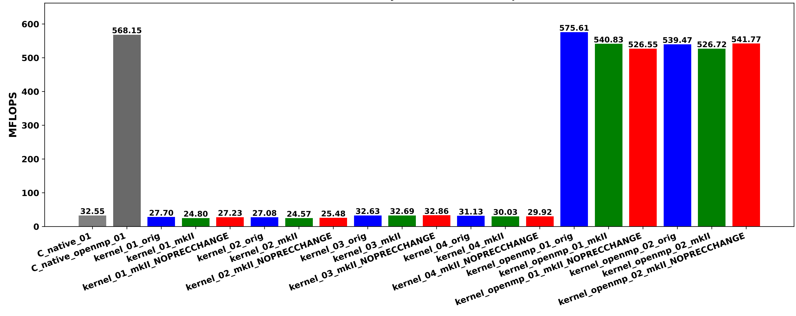
Rdot benchmark on Ryzen 3970X 32-Core (prec=512)
