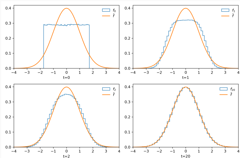
Figure 8: Convergence of the Invariant Distribution
