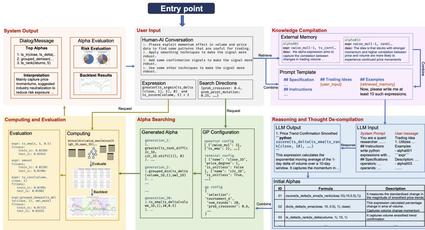
Figure 2: Alpha-GPT internal working pipeline: After a user inputs their ideas, the system goes into the knowledge compilation module.
