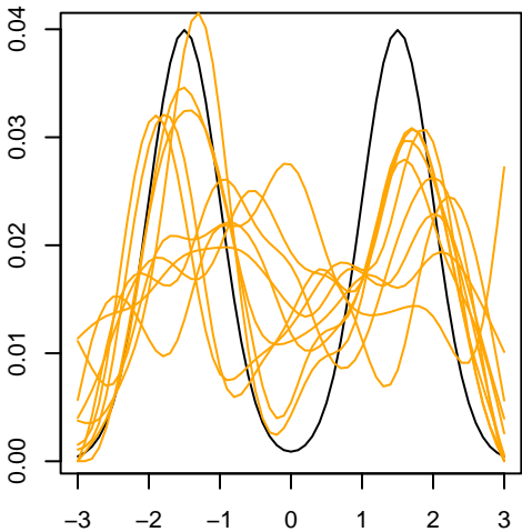
Langevin ( \eta.\phi=0.1 )
