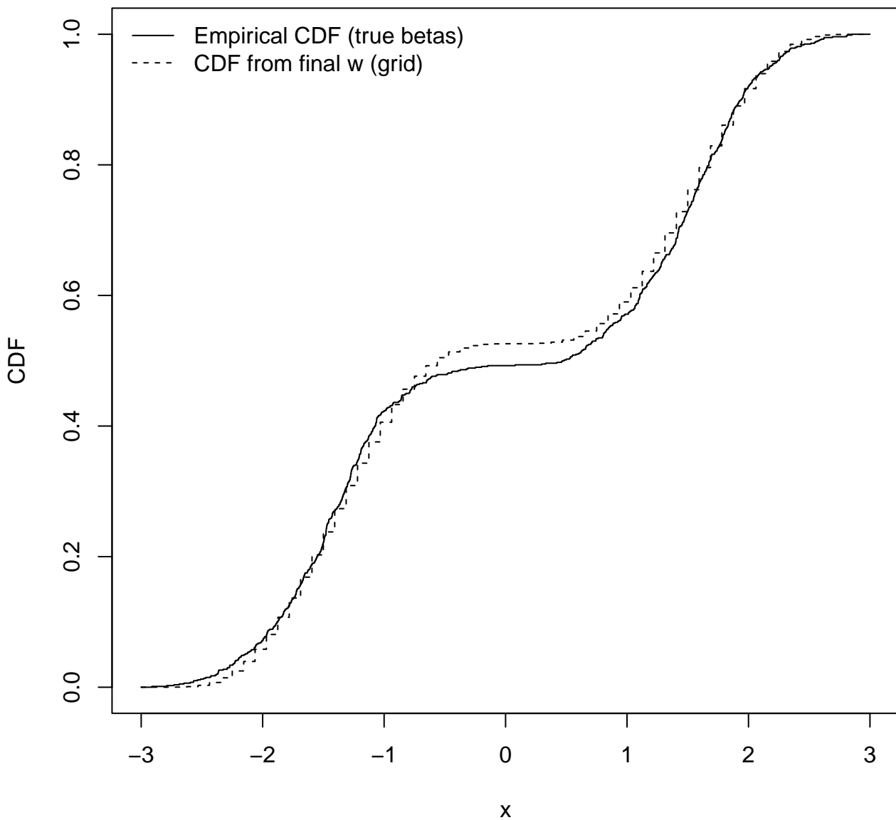
CDFs after 20000 iters (seed=8)
