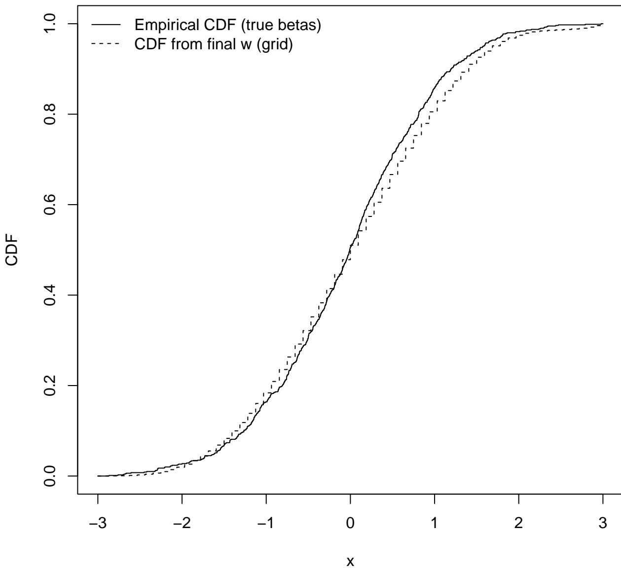
CDFs after 200000 iters (seed=1)
