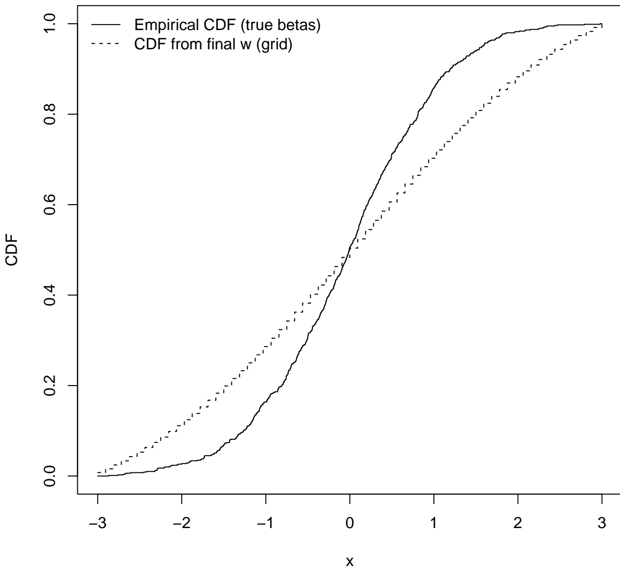
CDFs after 200 iters (seed=1)
