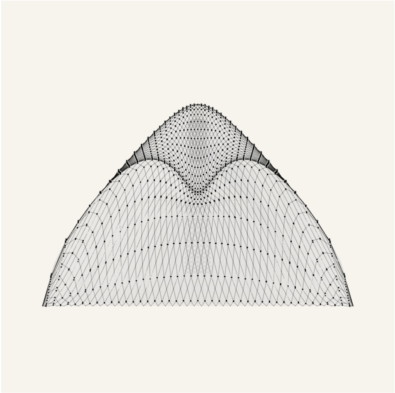
Figure 8. Candidate492 browser-rendered Front view for the same default state. This separate product camera compresses front depth, bounds the terminal lip contribution, depth-tests the pale grid against the lip, keeps rounded terminal width, and shows the center X-cell linkage through the projected cap rather than hiding mechanism state behind a pasted cap layer. The June 28 projection checkpoint remains open against the June 24 front reference.
