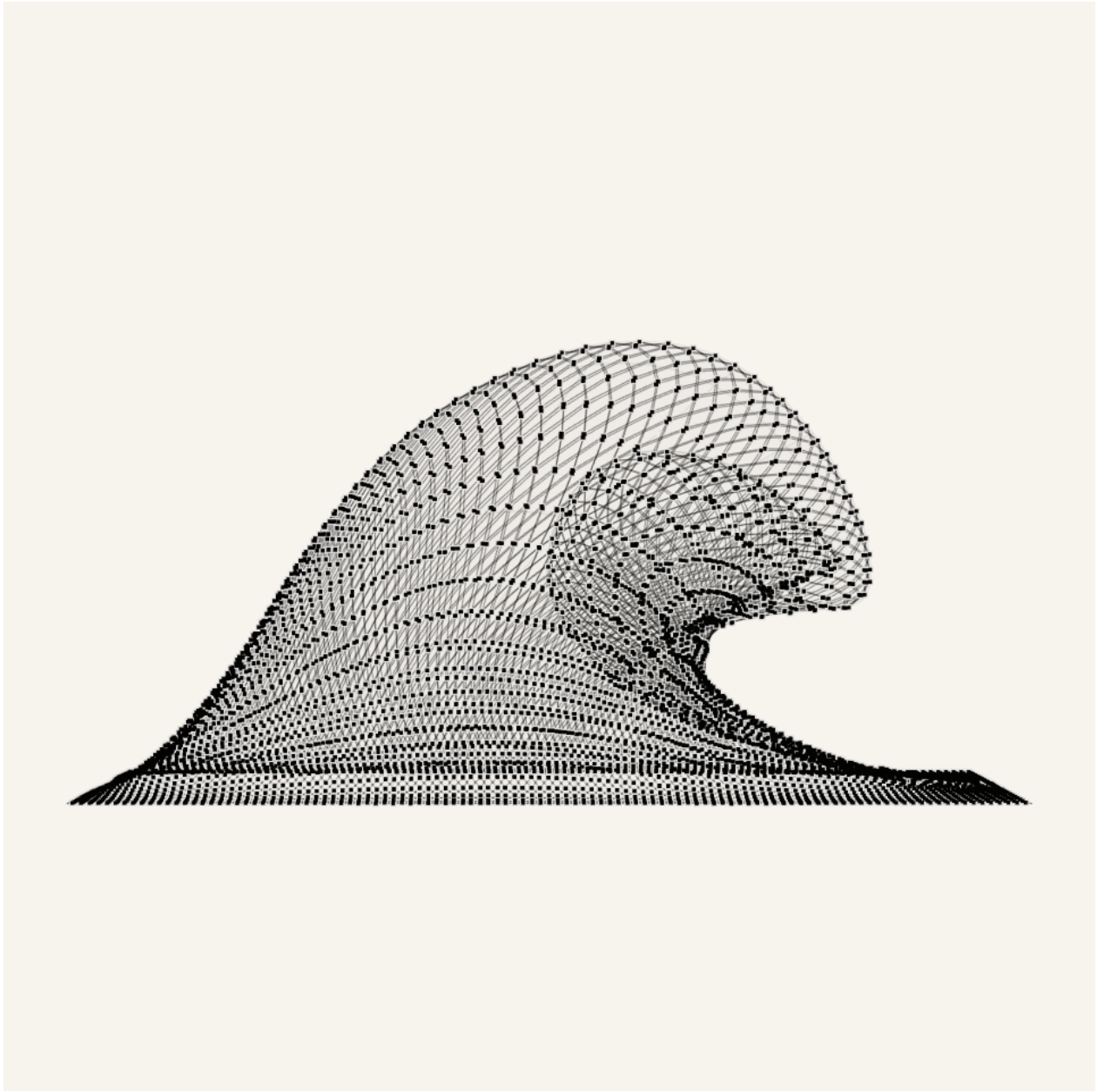
Figure 5. Candidate492 browser-rendered Side view for the default inverse-sheet state. The view is a full three-dimensional side camera with the readable surface, straight X-cell diagonals, center pivots, physical shared connector pins, and instanced shared-joint rods visible together. It preserves the open exact-match boundary: the underside remains readable and the between-cell joints stay explicit, but the reference-wave match is still not closed.
