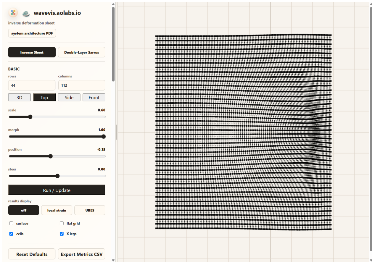
Figure 12. Candidate785 Top view with surface=0&connectors=1&cells=1. This proof view is intentionally dense because it shows the whole array through the X legs and cells layers. Each visible black square cell is the body for four straight legs, each opposite pair remains collinear/equal through the center, and adjacent cells meet at spherical two-use connector nodes. This is the current hard mechanism acceptance test, not a decorative overlay.
