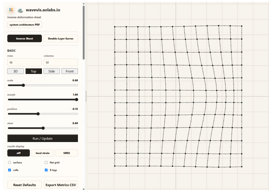
Figure 13. Candidate785 inspectable Top proof with rows=12, columns=12, surface=0, connectors=1, and cells=1. This low-density route exists so the hard cell contract can be inspected directly through the X legs and cells layers: a cell is not two nearby two-leg elements; it is one black square with four straight legs, opposite pairs are collinear and equal through the center, and each visible connector is a spherical node used by exactly two neighboring cells.
