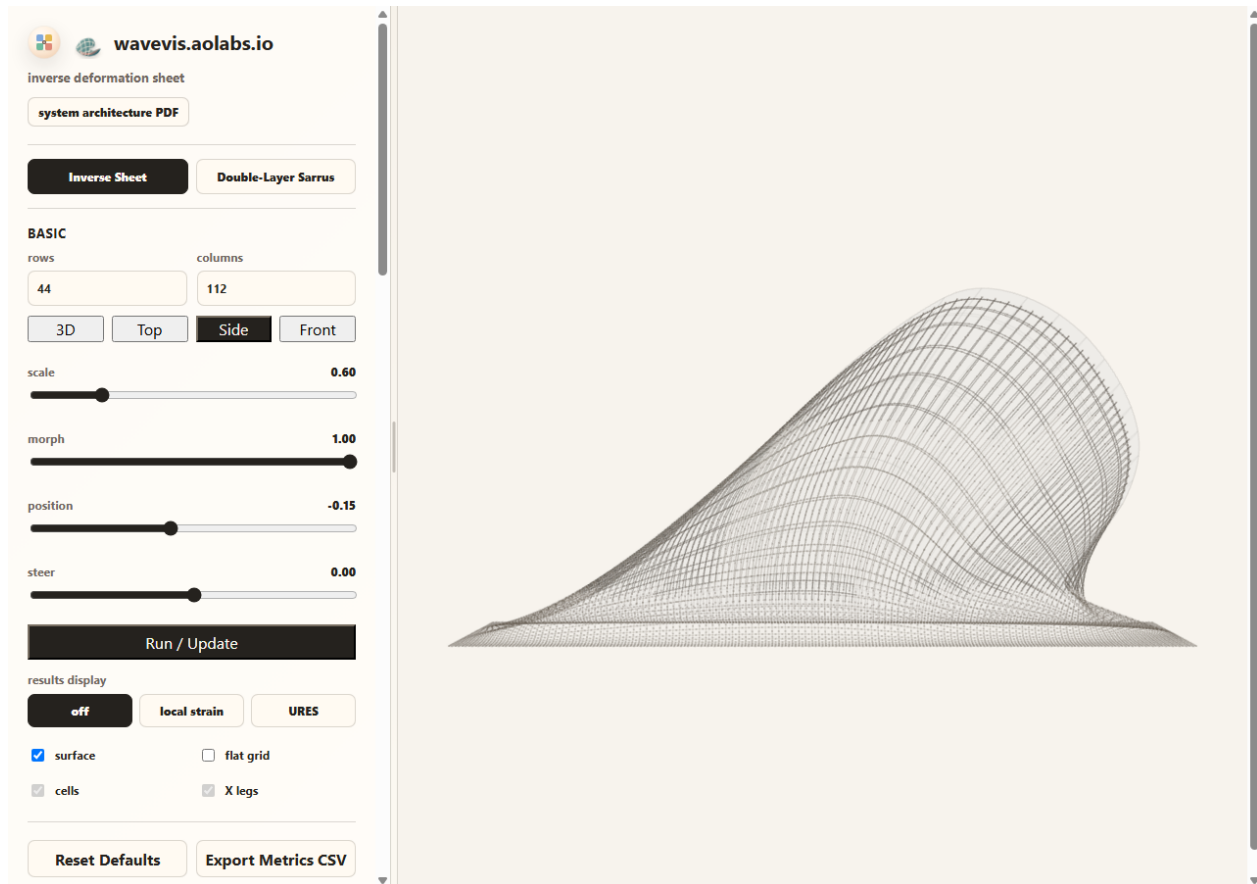
Figure 6. Candidate785 browser-rendered Side view from the live fallback route. The view keeps the readable surface subordinate to the actual mechanism: a lighter surface skin, muted X-cell ink, one-center/four-leg cell bodies, spherical two-use connector nodes, and visible shared-joint rods remain readable without forming a black silhouette mass. Candidate785 removes the dark under-overhang dimple Alan found in the public render by using the no-dimple side/isometric readable profile and open-throat lift. The underside now returns into the flat sheet instead of folding into a pocket, while the perimeter border band stays source-gated flat. The reference-wave match is still open: this checkpoint repairs the under-lip dimple and full-mechanism visibility floor, but it remains sparse and approximate rather than a completed Moana-like plunge.
