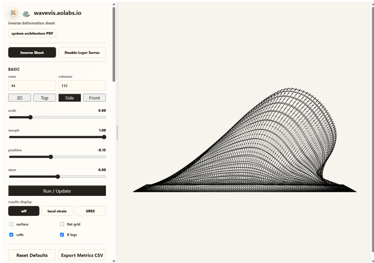
Figure 7. Candidate785 Side view with surface=0&connectors=1&cells=1. This X-only evidence removes the surface skin and shows the actual mechanism layer after the no-dimple side readable-profile split: each cell is one black square with four straight center-to-connector legs, opposite pairs are equal length and collinear through the cell center, and every connector is a spherical physical node with exactly two attached leg uses. Neighboring cells meet through visible connector nodes; no between-cell connector is allowed to become an X or a four-cell joint.
