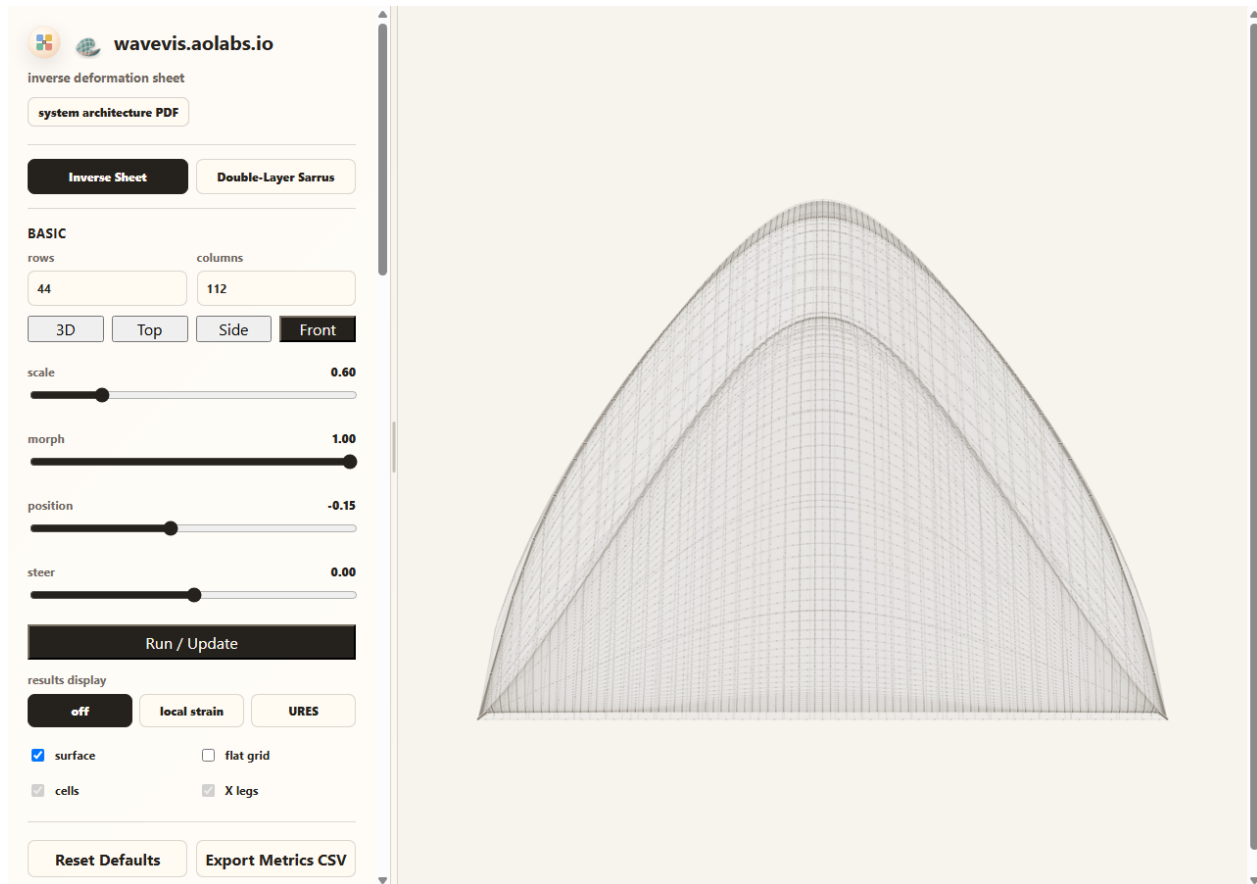
Figure 9. Candidate785 browser-rendered Front view retained as the separate spanwise product camera. This view compresses front depth, bounds the terminal lip contribution, depth-tests the pale grid against the lip, keeps rounded terminal width, and shows the black-square X-cell linkage with spherical connector nodes through the projected cap rather than hiding mechanism state behind a pasted cap layer. The projection checkpoint remains open against the June 24 and June 28 references.
