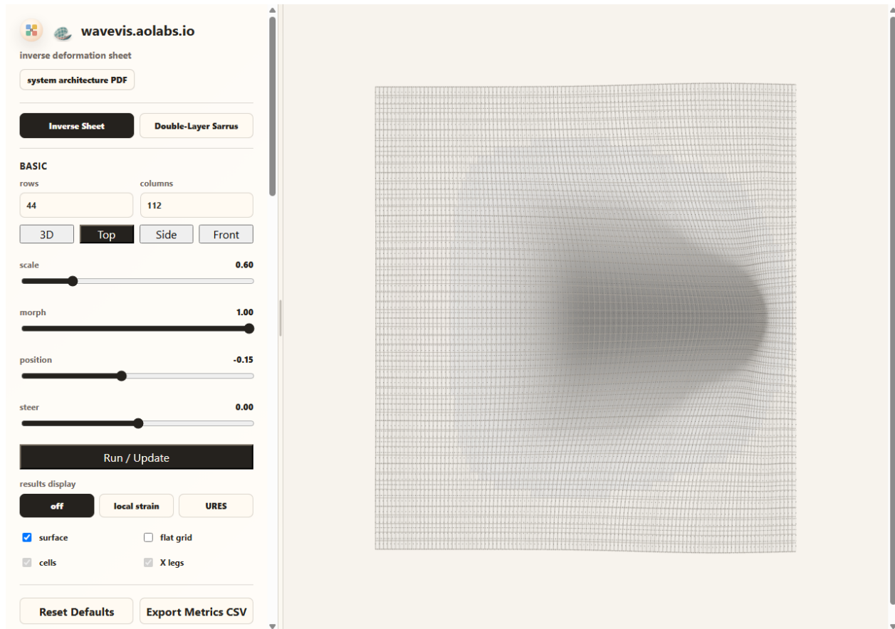
Figure 10. Candidate785 browser-rendered Top view for the same default state. The surface-plus-X view keeps the rounded proof profile rather than inheriting the side-only no-dimple profile, and it uses a stronger reference-sheet grid, one continuous black-square/four-leg X layer, real center-to-connector rods, spherical connector nodes, a guarded mid-section oval term, and a bounded height-shadow from the readable surface. Strict surface=0&connectors=1&cells=1 top inspection still exposes the collinear equal-pair X-only mechanism rather than hiding it, and the top footprint remains an open visual-match target rather than a solved reference state.
