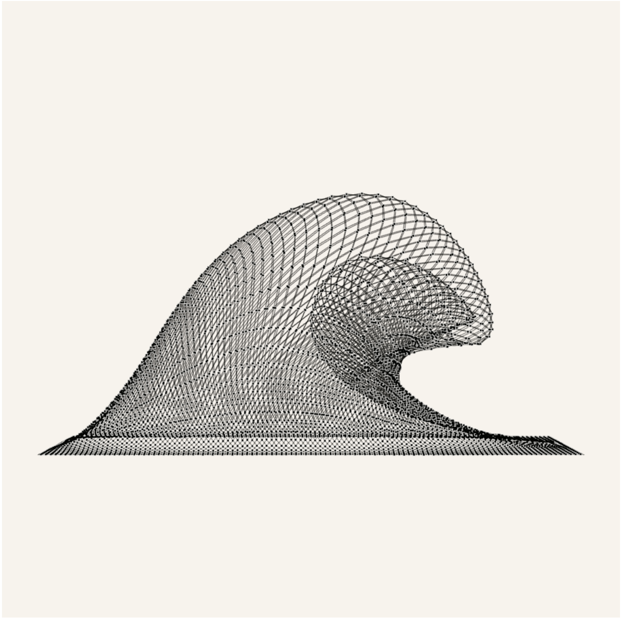
Figure 6. Candidate492 Side view with surface=0&connectors=1 . This X-only evidence removes the surface skin and shows the actual mechanism layer: each cell is a straight two-bar X, each diagonal is bisected at the center pivot, and neighboring cells meet at visible shared connector pins through real center-to-connector rods.
